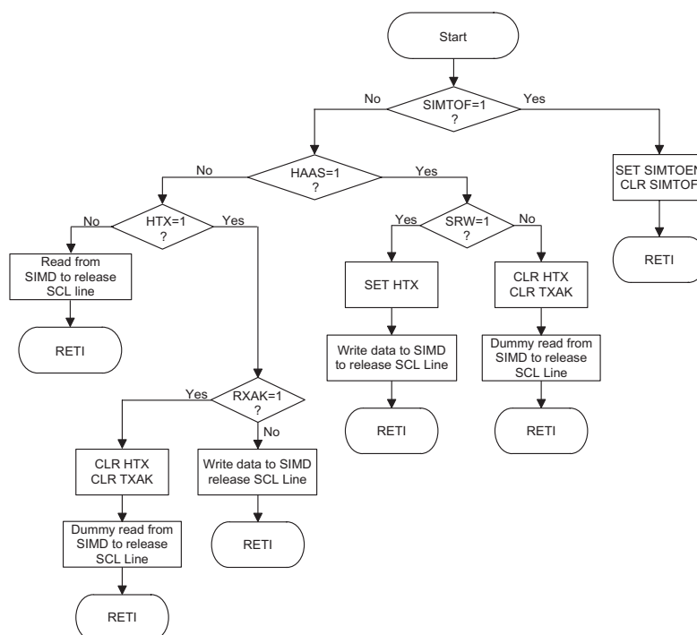
I²C Bus ISR Flow Chart
