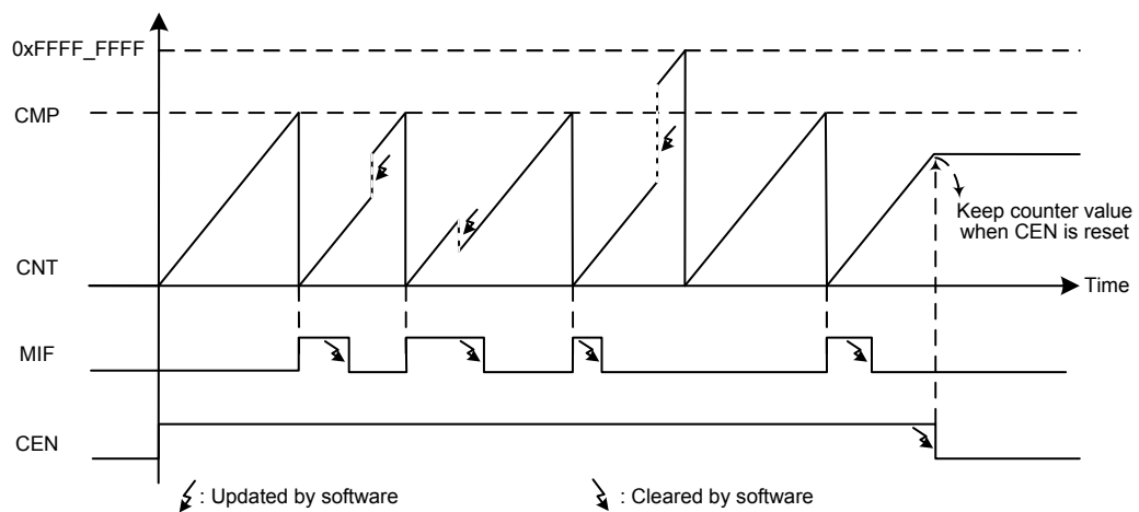
Figure 70. BFTM – Repetitive Mode
