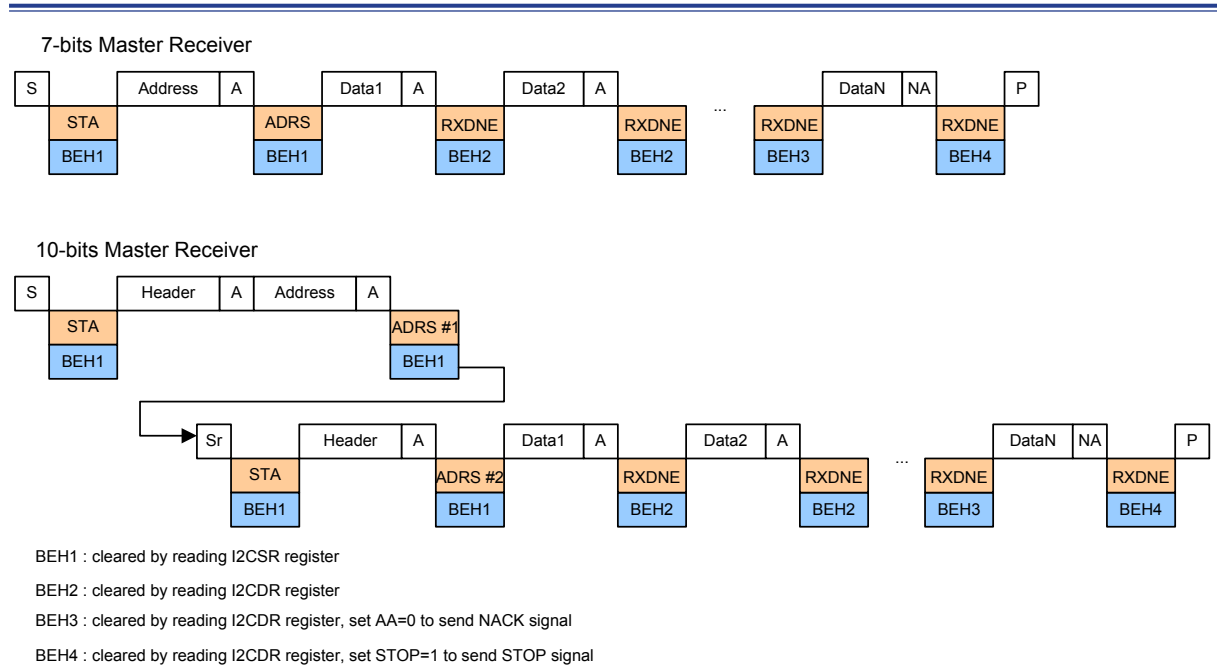
Figure 146. Master Receiver Timing Diagram
