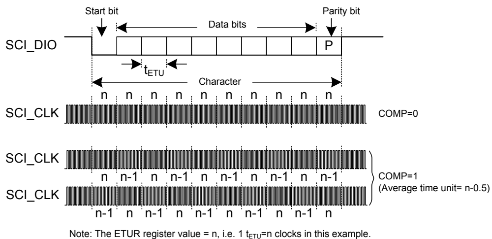
Figure 175. Character Frame and Compensation Mode
