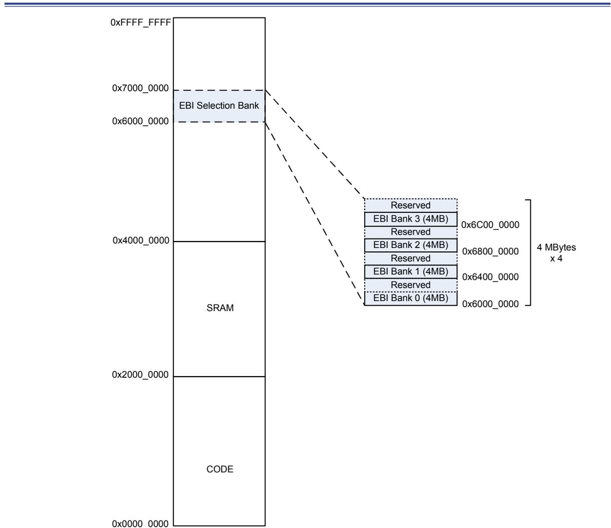
Figure 198. EBI Bank Memory Map
