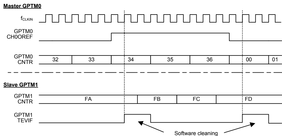
Figure 65. Pausing GPTM1 using the GPTM0 CH0OREF Signal
