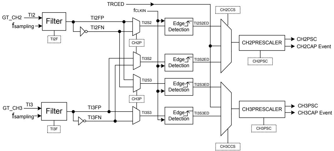
Figure 51. Channel 2 and Channel 3 Input Stages
