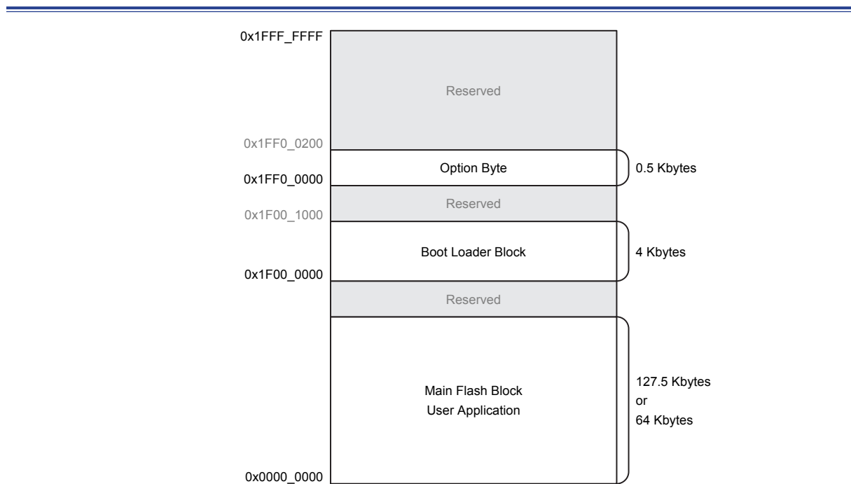
Figure 6. Flash Memory Map
