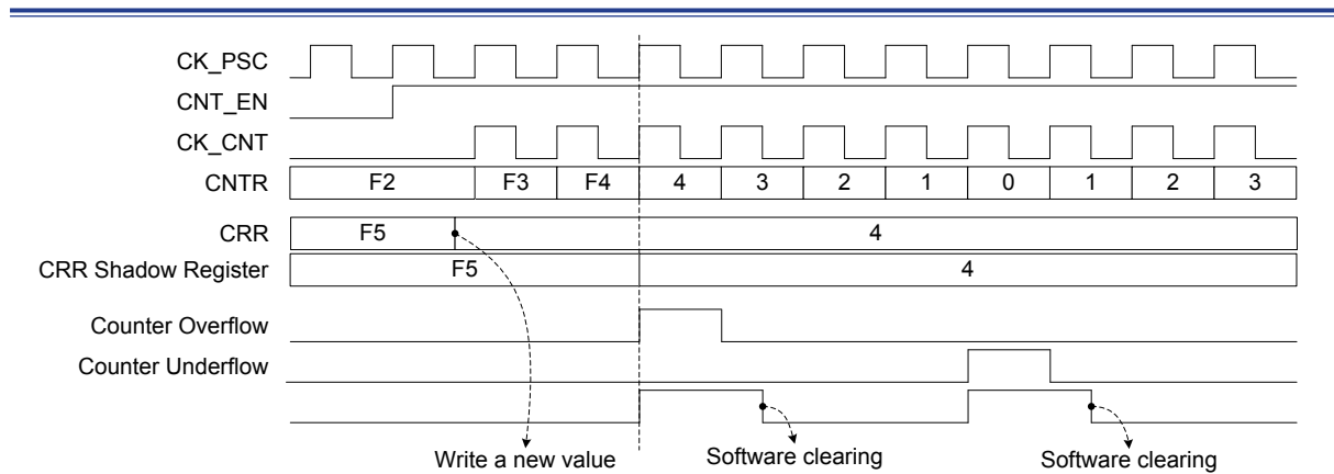
Figure 76. Center-aligned Counting Example
