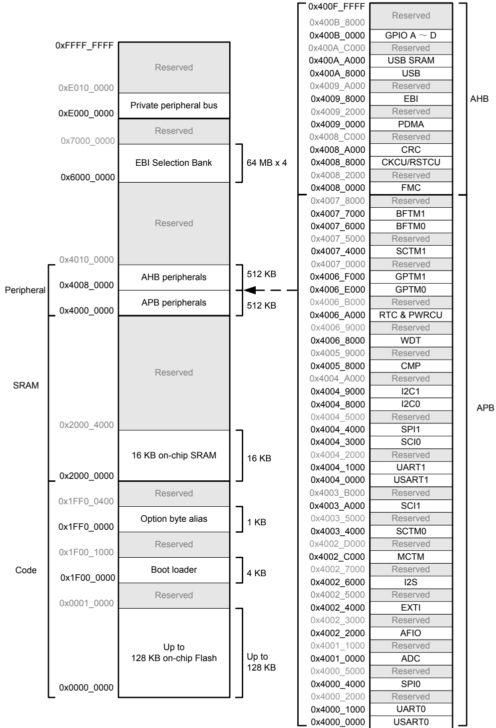
Figure 4. Memory Map
