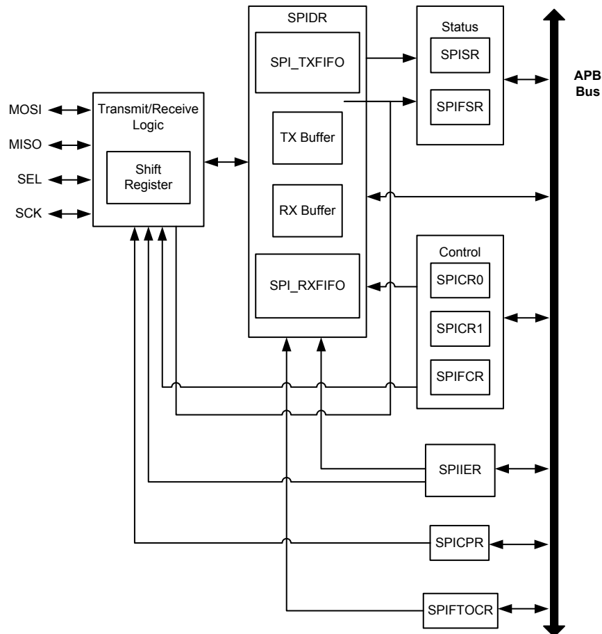
Figure 150. SPI Block Diagram
