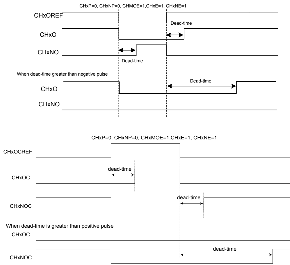
Figure 98. Dead-time Insertion Performed for Complementary Outputs
