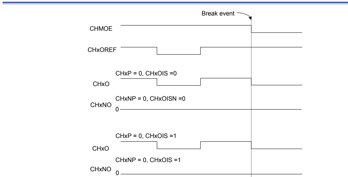
Figure 104. Hardware Protection When Both CHxO and CHxNO Are in Active Condition
