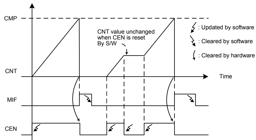
Figure 71. BFTM – One Shot Mode
