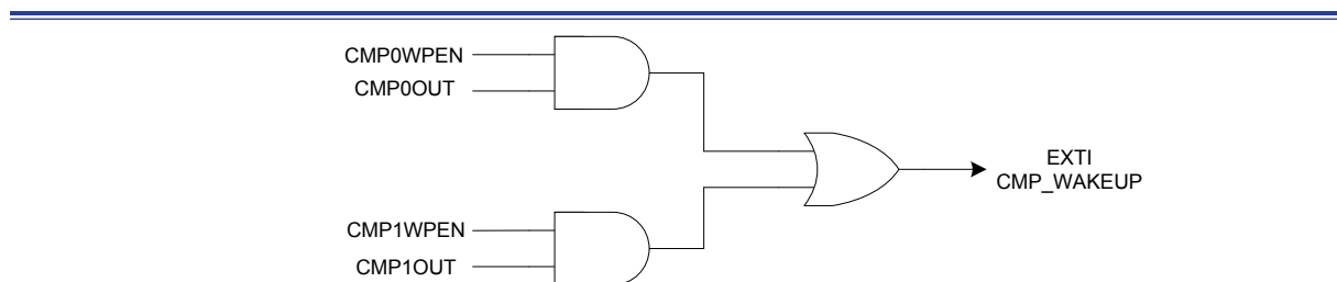
Figure 34. Wakeup Signals of Comparators
