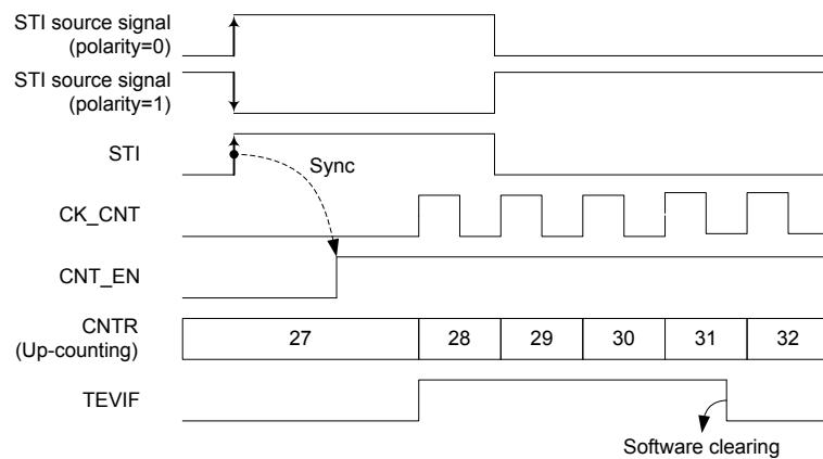
Figure 44. GPTM in Trigger Mode
