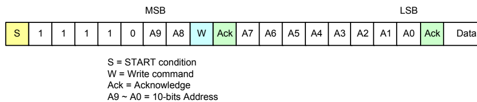
Figure 140. 10-bit Addressing Write Transmit Mode
