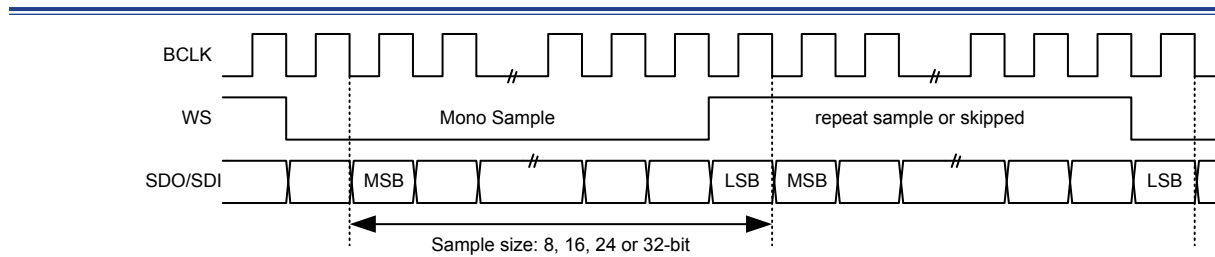
Figure 214. I 2 S-justified Repeat Mode Waveforms
