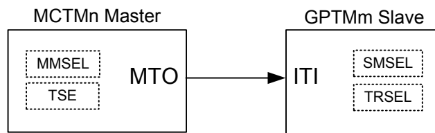
Figure 84. Master MCTMn and Slave GPTMm Connection
