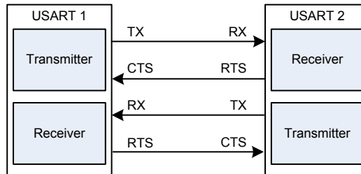
Figure 163. Hardware Flow Control between 2 USARTs
