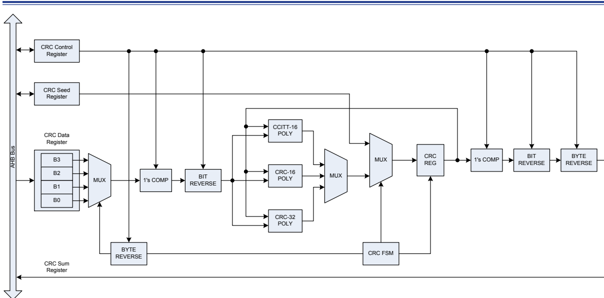
Figure 217. CRC Block Diagram
