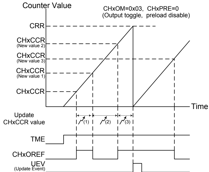
Figure 56. Toggle Mode Channel Output Reference Signal (CHxPRE = 0)
