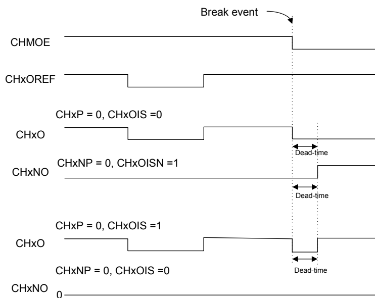
Figure 103. Channel 0 ~ 2 Only One Output Enabled when Fault Event Occurs
