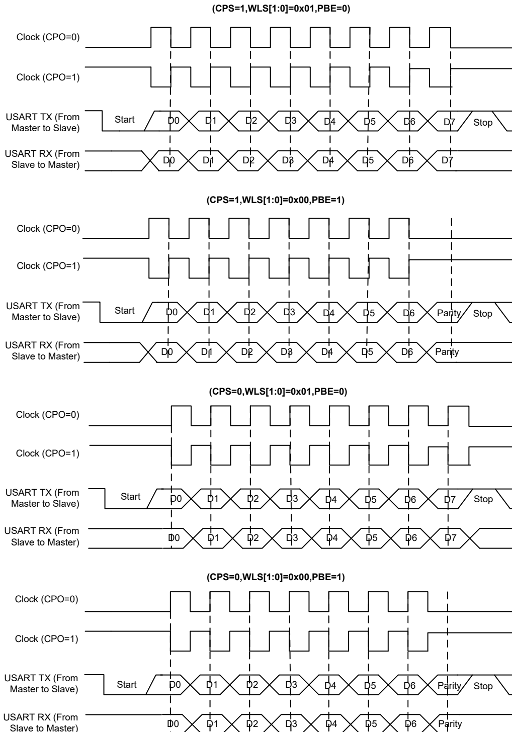
Figure 170. 8-bit Format USART Synchronous Waveform
