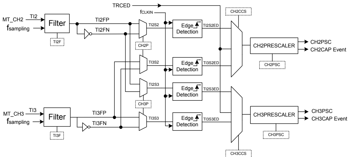
Figure 90. Channel 2 and Channel 3 Input Stages
