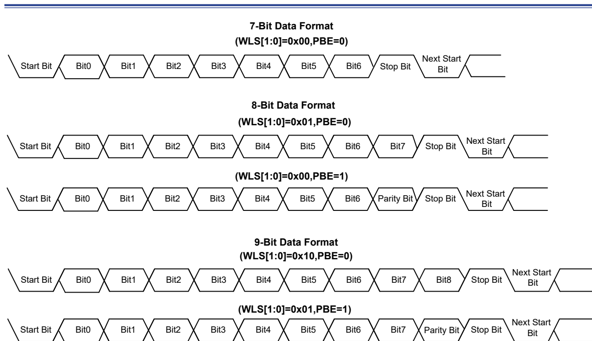
Figure 161. USART Serial Data Format
