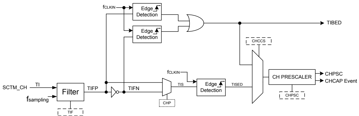
Figure 126. Channel Input Stages
