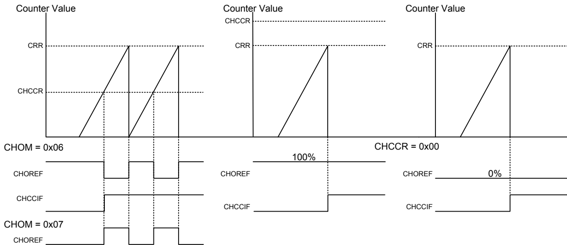
Figure 131. PWM Mode Channel Output Reference Signal
