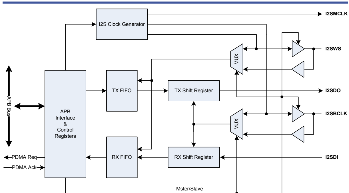
Figure 199. I 2 S Block Diagram
