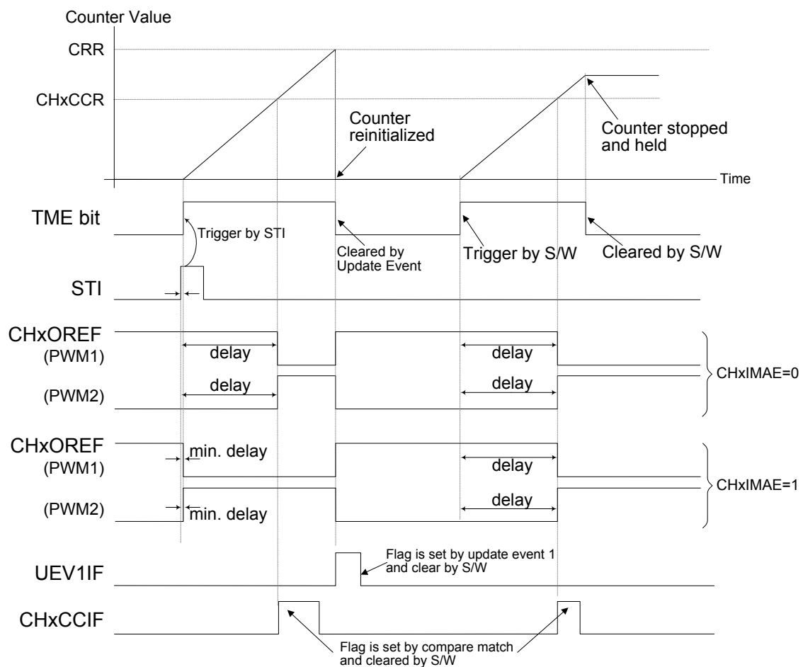
Figure 108. Single Pulse Mode
