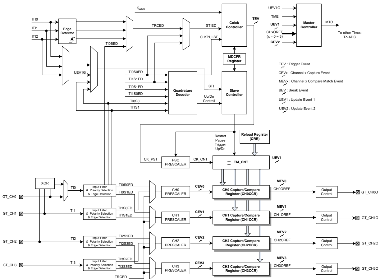
Figure 35. GPTM Block Diagram
