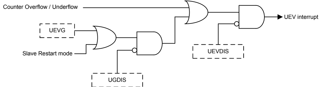
Figure 132. Update Event Setting Diagram
