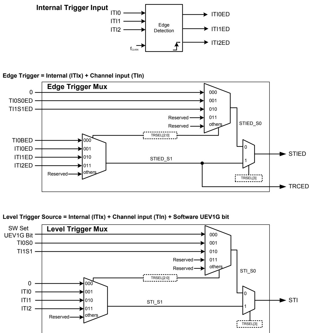
Figure 40. Trigger Controller Block
