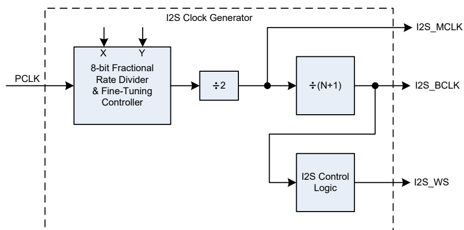
Figure 201. I 2 S Clock Generator Diagram
