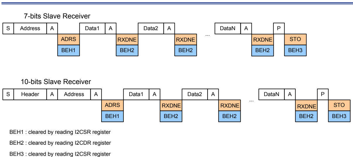
Figure 148. Slave Receiver Timing Diagram
