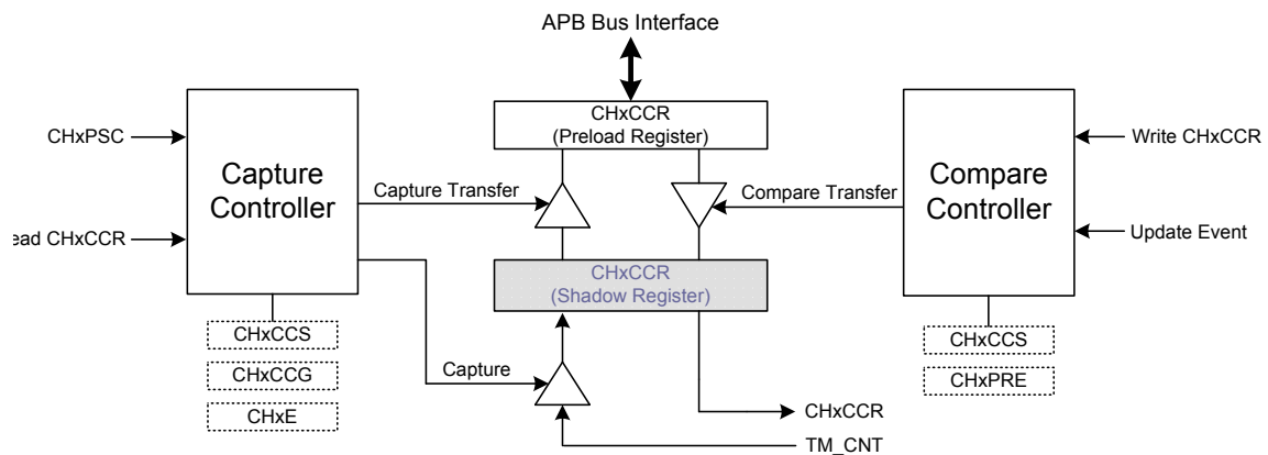
Figure 47. Capture/Compare Block Diagram
