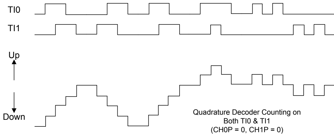
Figure 54. Both TI0 and TI1 Quadrature Decoder Counting
