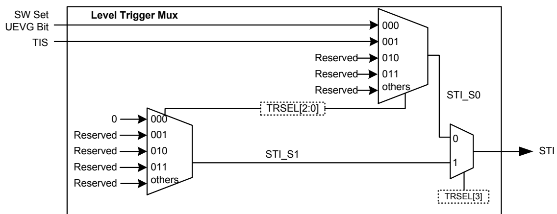
Figure 119. Trigger Controller Block
