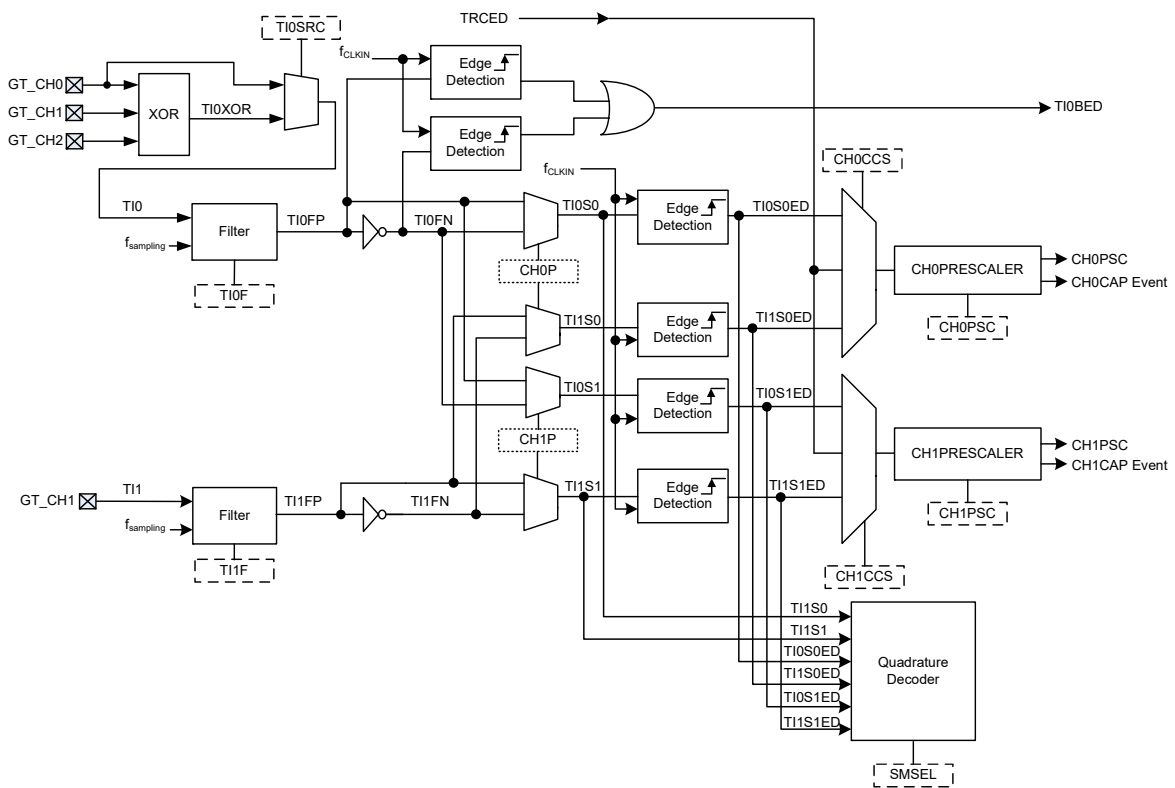
Figure 53. Input Stage and Quadrature Decoder Block Diagram
