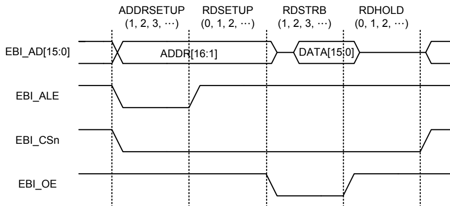
Figure 192. EBI Multiplexed 16-bit Data, 16-bit Address Read Operation
