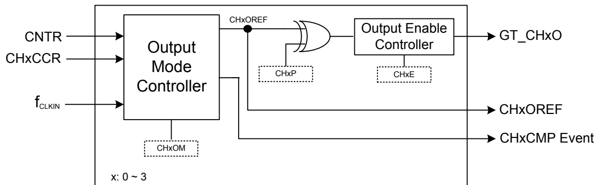
Figure 55. Output Stage Block Diagram
