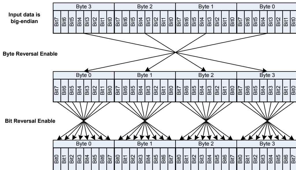
Figure 218. CRC Data Bit and Byte Reversal Example
