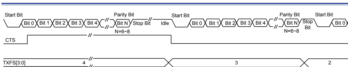
Figure 165. USART CTS Flow Control
