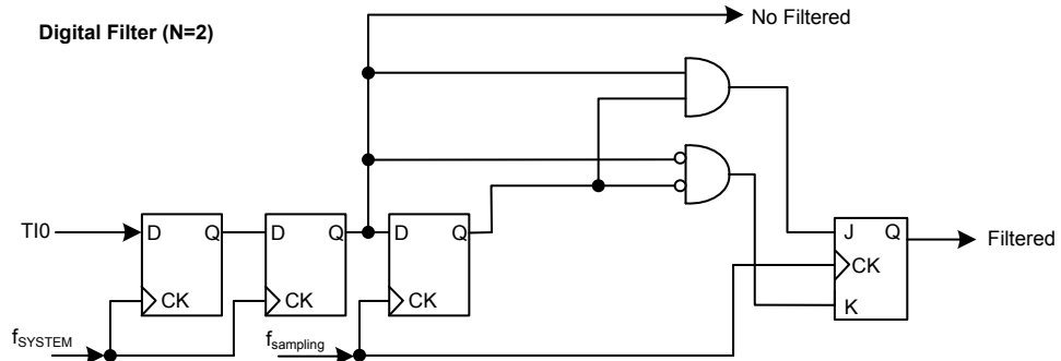
Figure 91. TIO Digital Filter Diagram with N = 2
