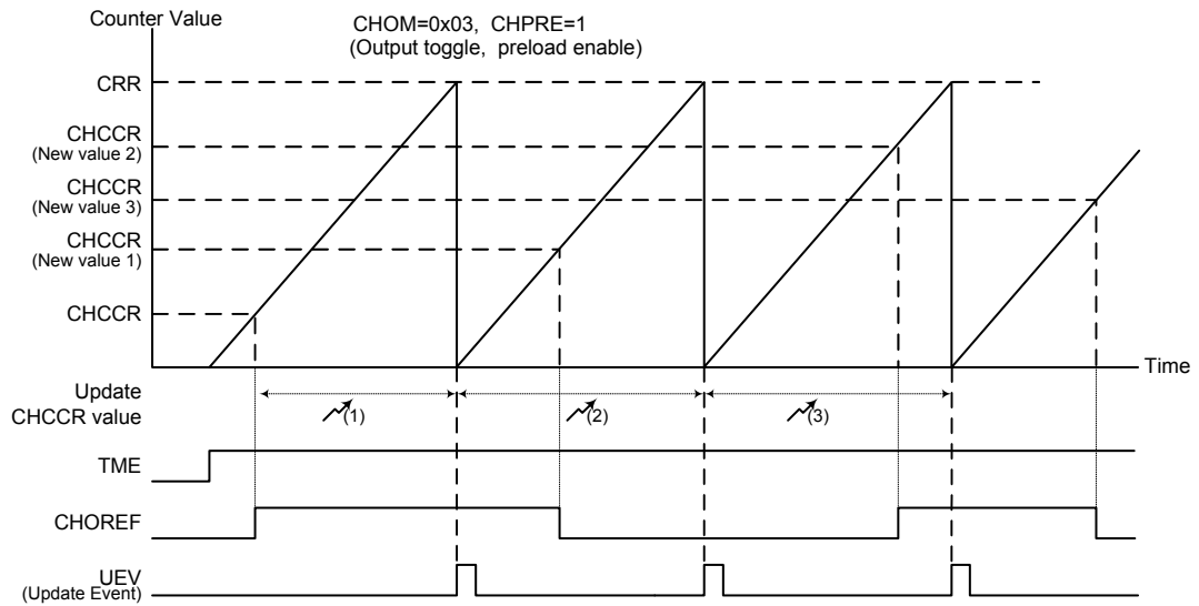
Figure 130. Toggle Mode Channel Output Reference Signal (CHPRE = 1)
