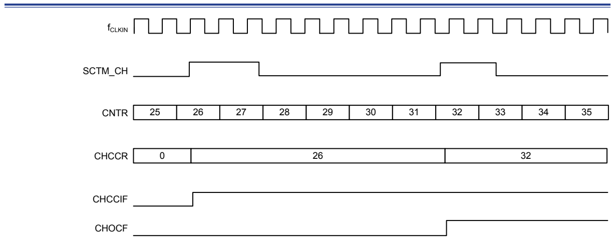
Figure 125. Input Capture Mode
