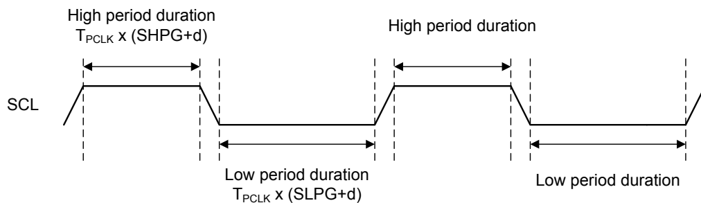
Figure 149. SCL Timing Diagram
