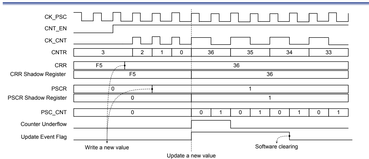
Figure 37. Down-counting Example
