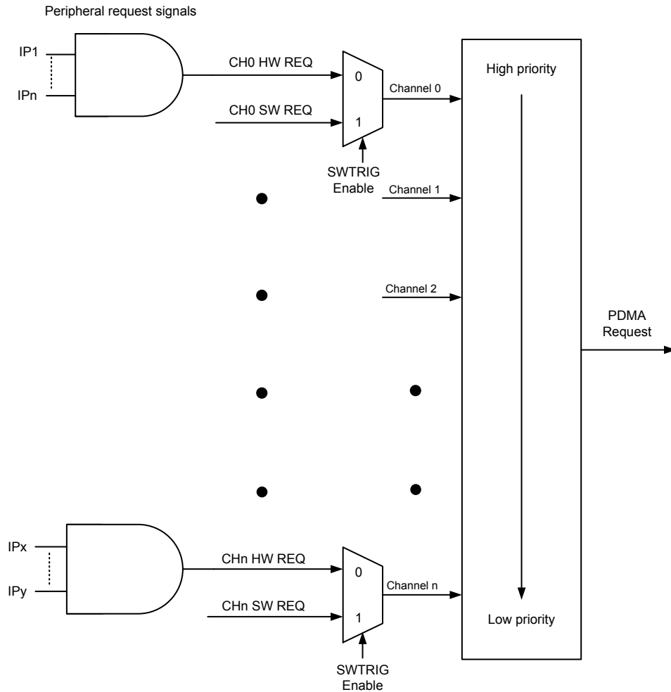
Figure 184. PDMA Request Mapping Architecture
