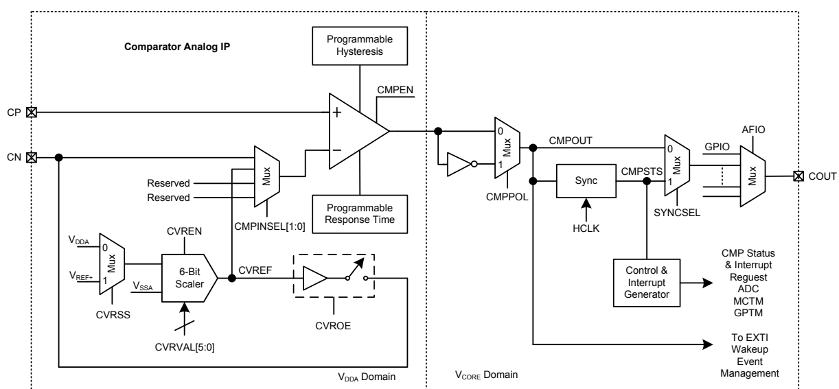
Figure 31. Comparator Block Diagram
