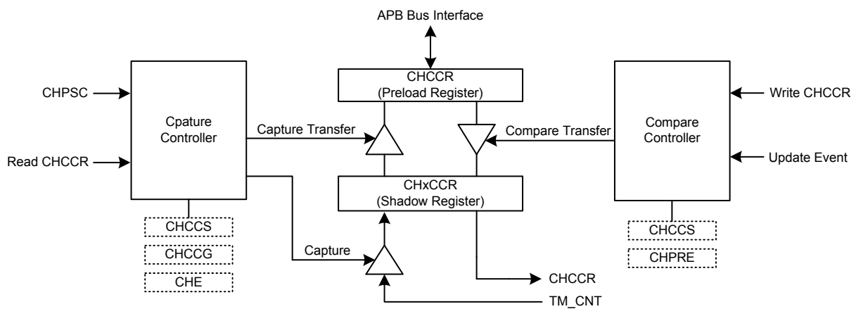
Figure 124. Capture/Compare Block Diagram
