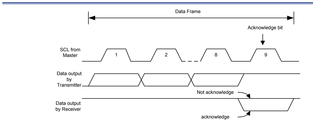
Figure 142. I 2 C Bus Acknowledge
