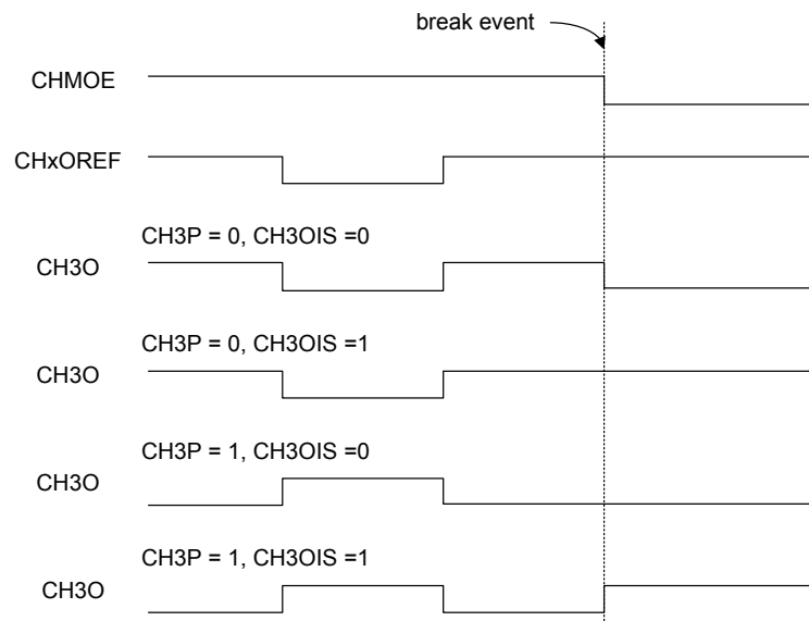
Figure 101. Channel 3 Output with a Break Event Occurrence
