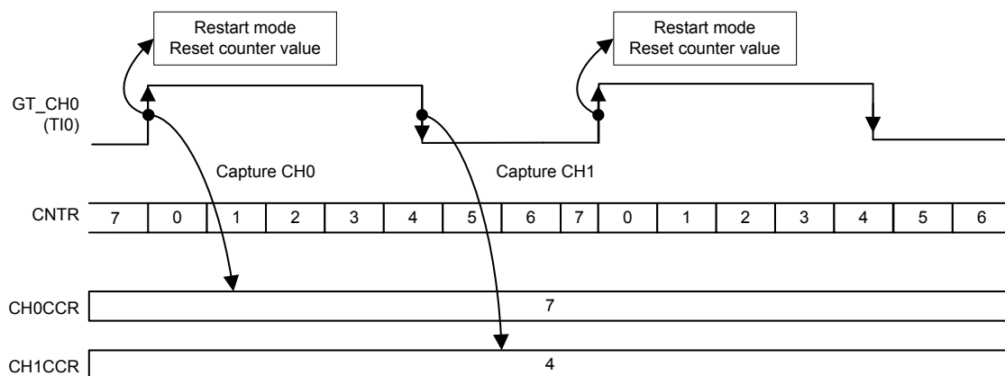
Figure 49. PWM Pulse Width Measurement Example
