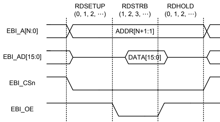
Figure 189. EBI Non-multiplexed 16-bit Data, N-bit Address Read Operation
