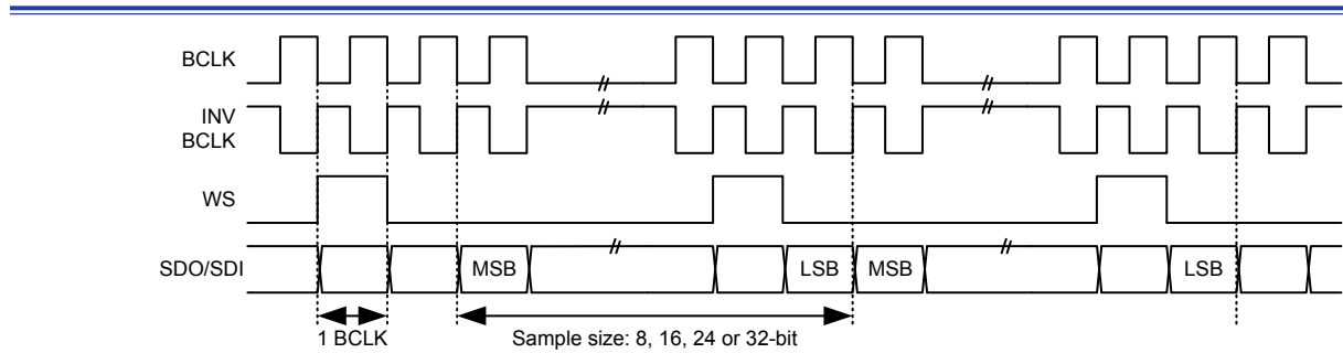
Figure 208. I 2 S-justified Mono Mode Waveforms
