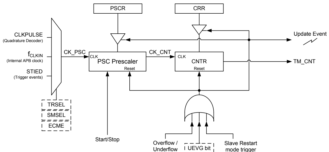
Figure 39. GPTM Clock Selection Source
