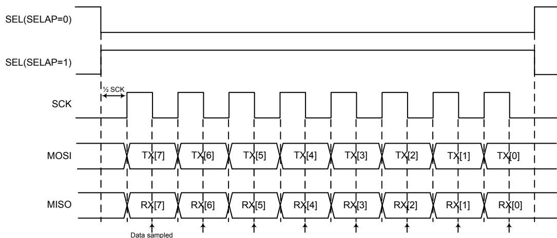
Figure 153. SPI Single Byte Transfer Timing Diagram – CPOL = 0, CPHA = 1
