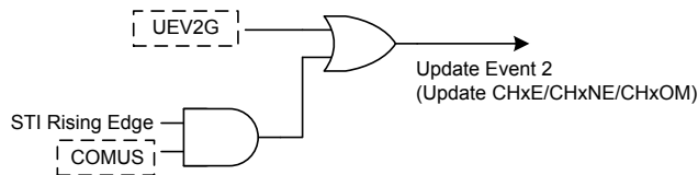
Figure 107. Update Event 2 Setup Diagram
