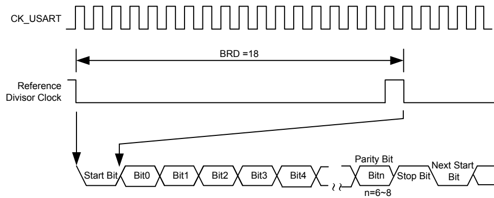
Figure 162. USART Clock CK_USART and Data Frame Timing
