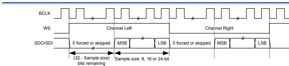
Figure 207. Right-justified Stereo Mode Waveforms (32-bit Channel Enabled)
