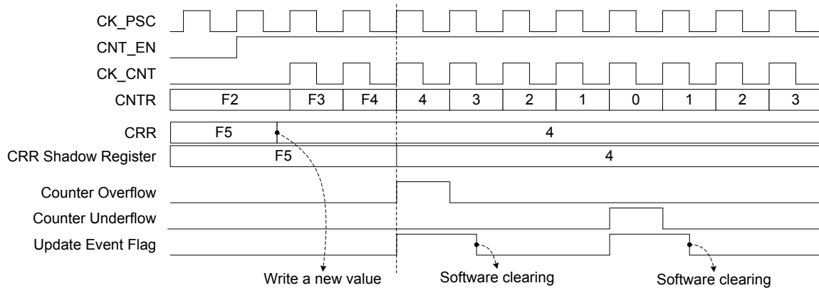
Figure 38. Center-aligned Counting Example
