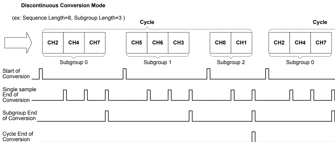
Figure 30. Discontinuous Conversion Mode
