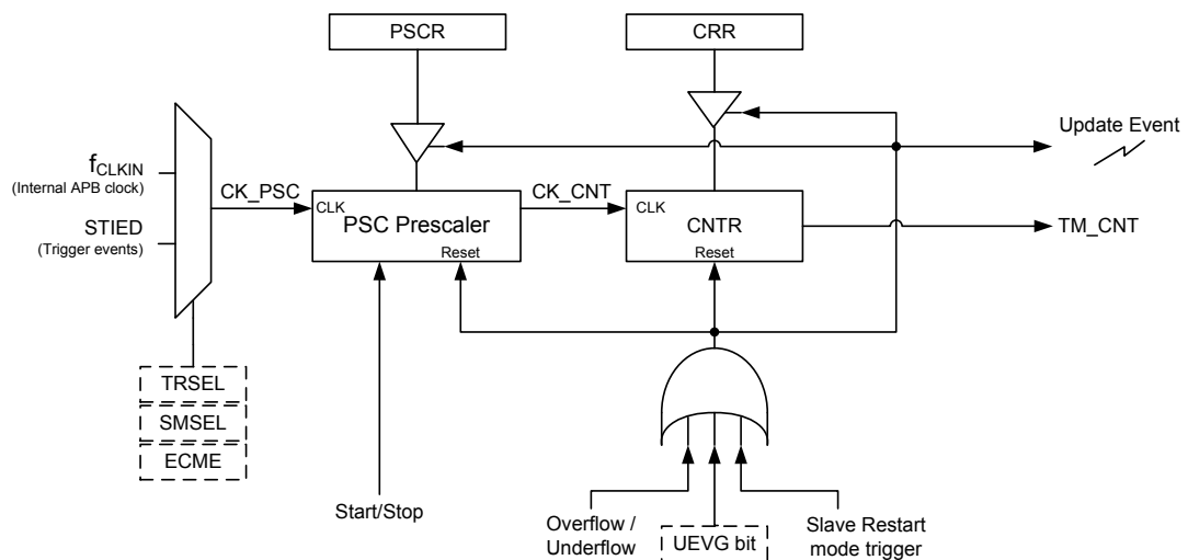
Figure 118. SCTM Clock Selection Source
