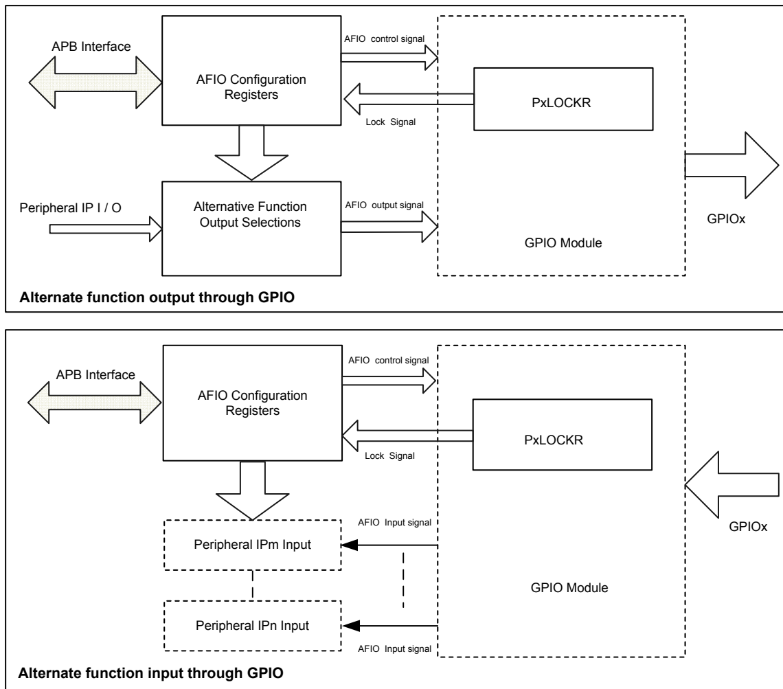
Figure 22. AFIO Block Diagram
