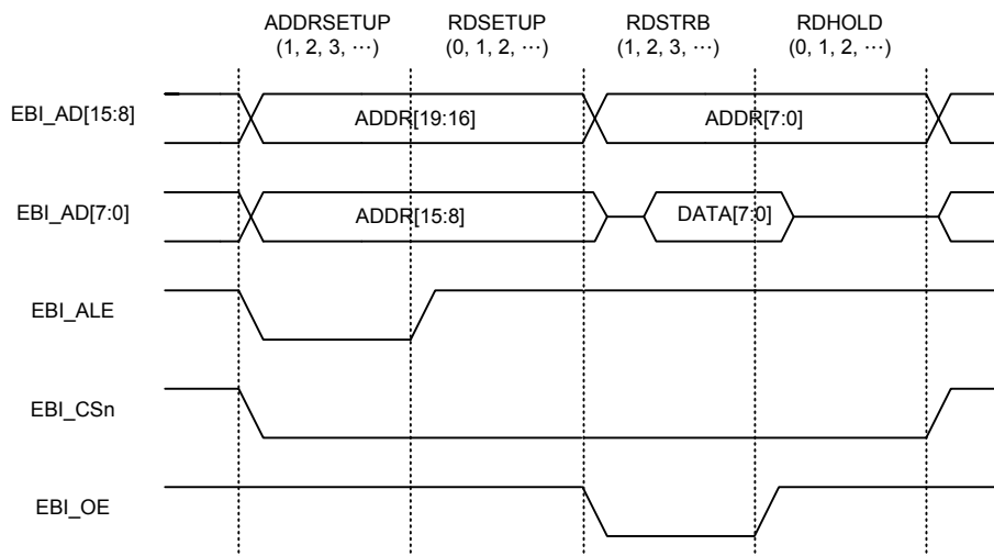
Figure 194. EBI Multiplexed 8-bit Data, 20-bit Address Read Operation
