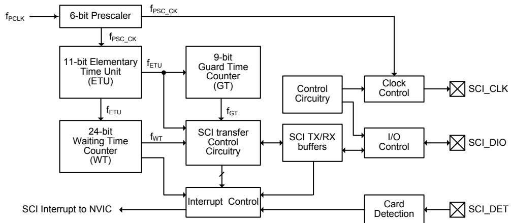
Figure 174. SCI Block Diagram
