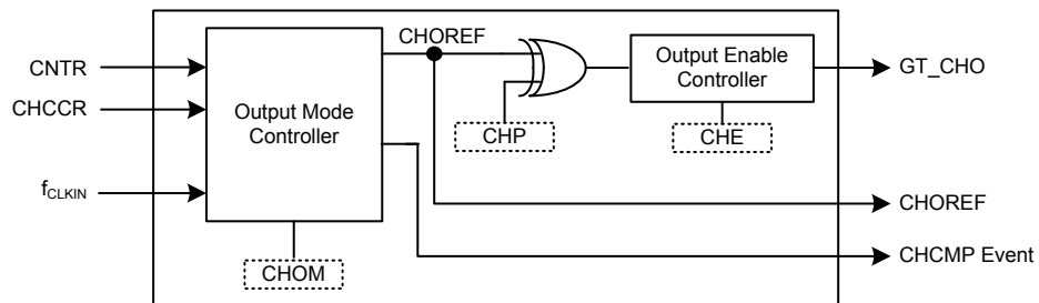
Figure 128. Output Stage Block Diagram
