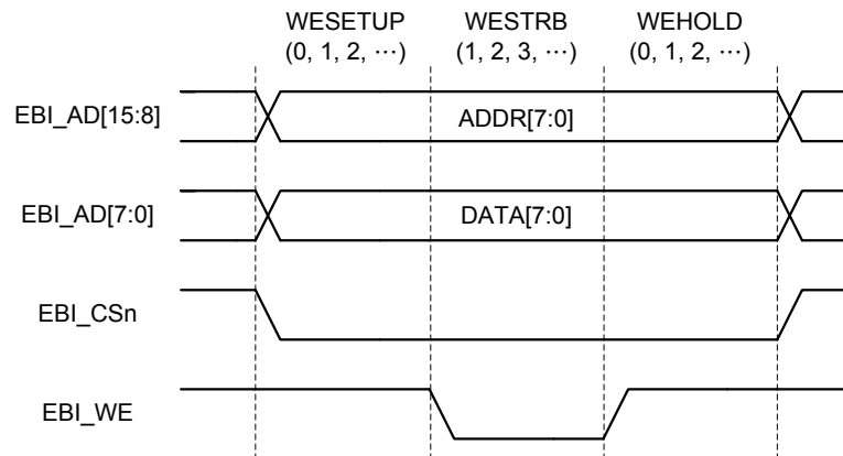
Figure 188. EBI Non-multiplexed 8-bit Data, 8-bit Address Write Operation
