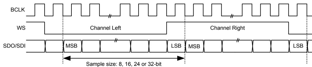
Figure 202. I 2 S-justified Stereo Mode Waveforms
