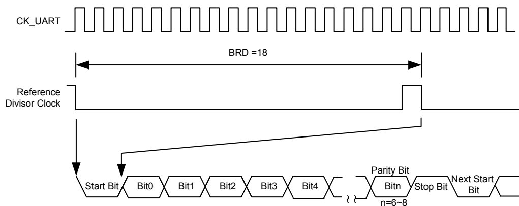
Figure 173. UART Clock CK_UART and Data Frame Timing
