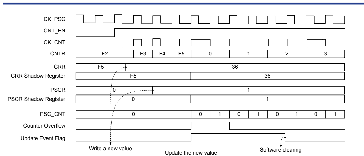
Figure 36. Up-counting Example
