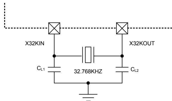
Figure 17. External Crystal, Ceramic, and Resonators for LSE
