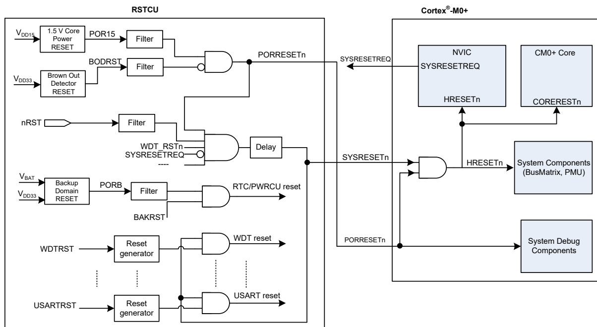
Figure 18. RSTCU Block Diagram
