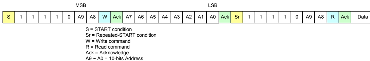
Figure 141. 10-bit Addressing Read Receive Mode
