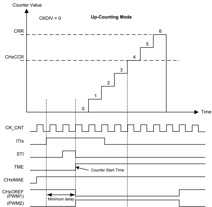
Figure 63. Immediate Active Mode Minimum Delay
