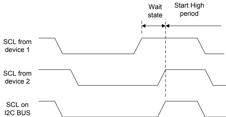
Figure 143. Clock Synchronization during Arbitration
