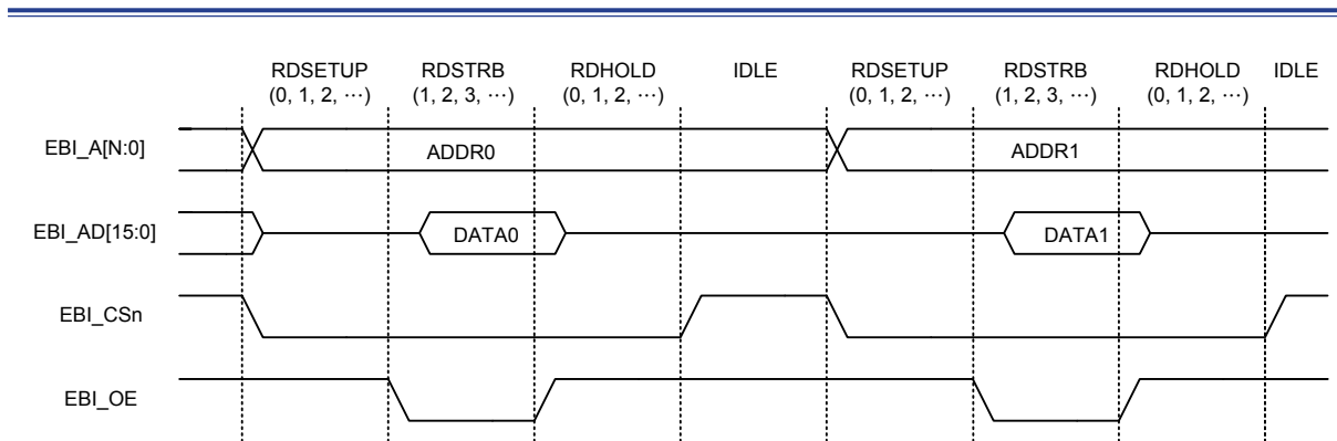
Figure 196. EBI Inserts an IDLE Cycle between Transactions in the Same Bank (NOIDLE = 0)
