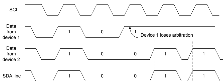
Figure 144. Two Master Arbitration Procedure
