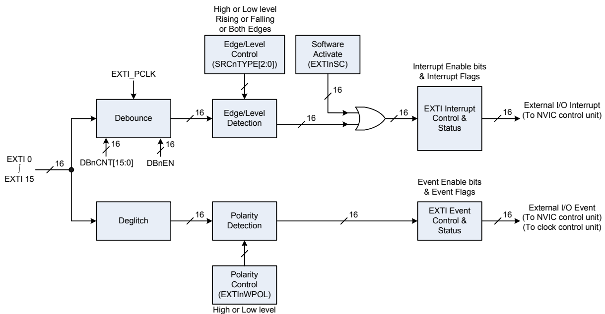
Figure 24. EXTI Block Diagram
