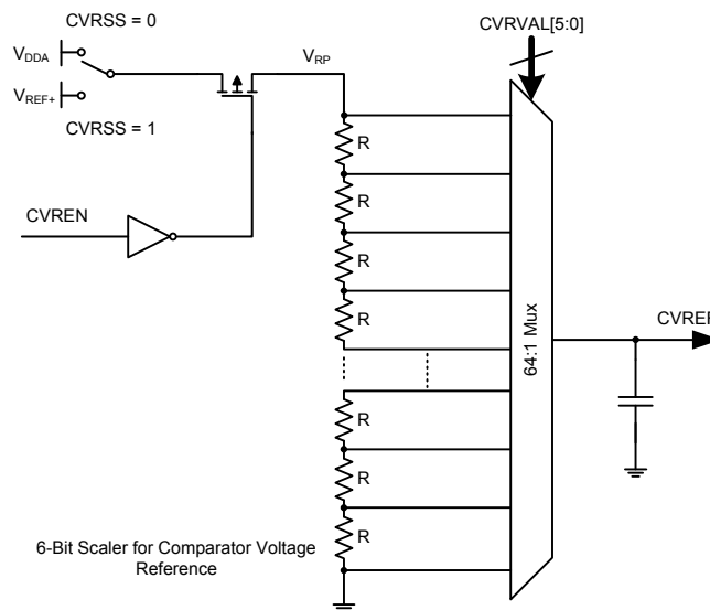
Figure 32. 6-Bit Scaler for Comparator Voltage Reference Block Diagram
