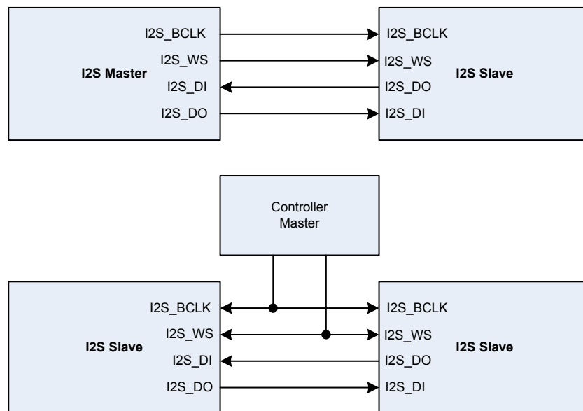
Figure 200. Simple I 2 S Master/Slave Configuration
