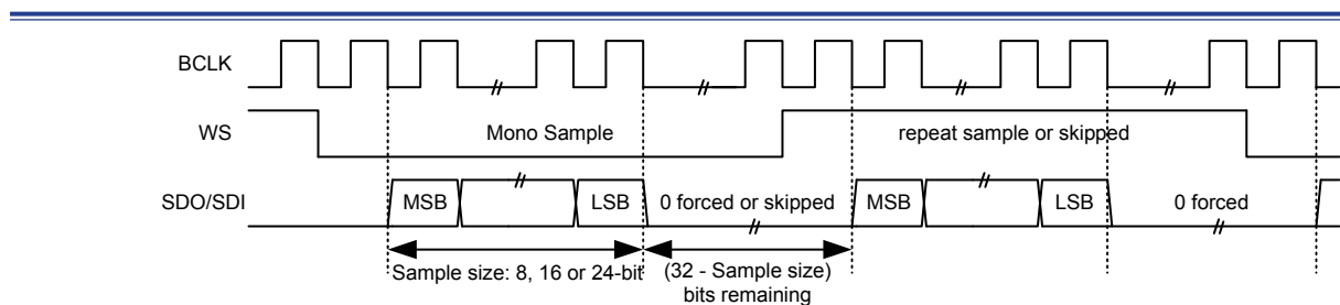
Figure 215. I 2 S-justified Repeat Mode Waveforms (32-bit Channel Enabled)
