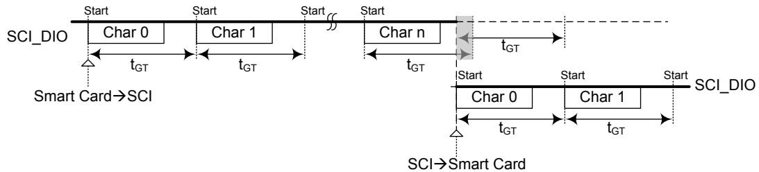
Figure 176. Guard Time Duration
