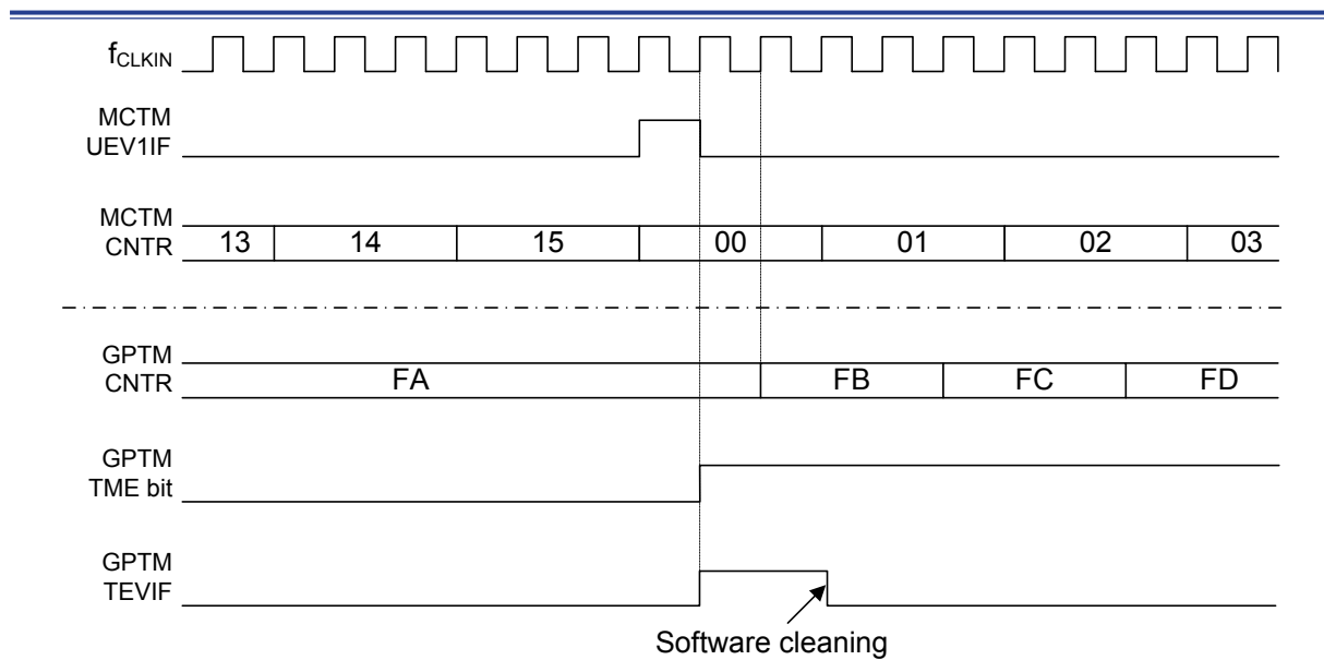
Figure 112. Triggering GPTM with MCTM Update Event 1
