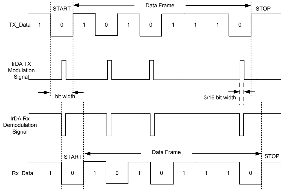
Figure 166. IrDA Modulation and Demodulation
