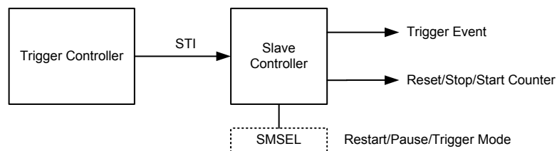
Figure 80. Slave Controller Diagram
