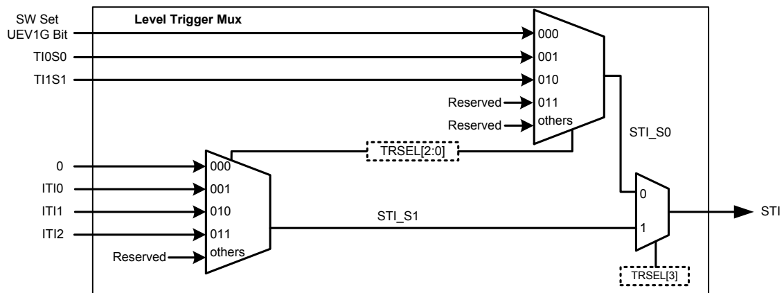
Figure 79. Trigger Controller Block
