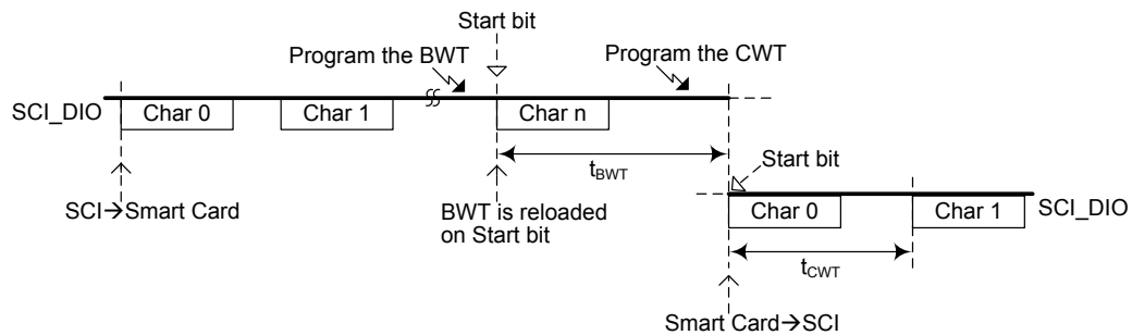
Figure 177. Character and Block Waiting Time Duration – CWT and BWT
