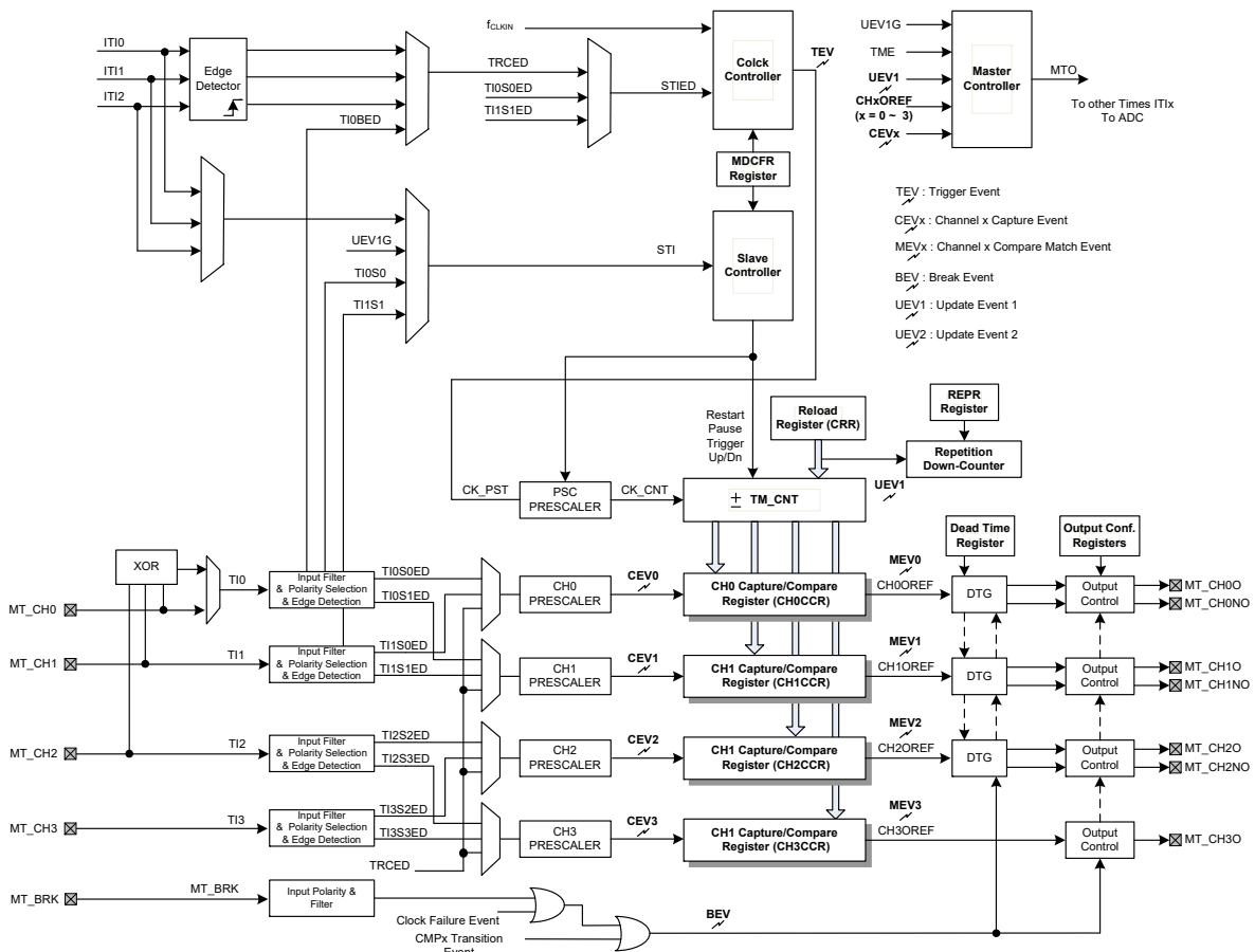
Figure 73. MCTM Block Diagram
