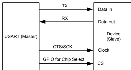
Figure 169. USART Synchronous Transmission Example
