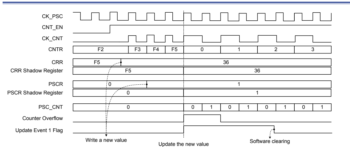
Figure 74. Up-counting Example
