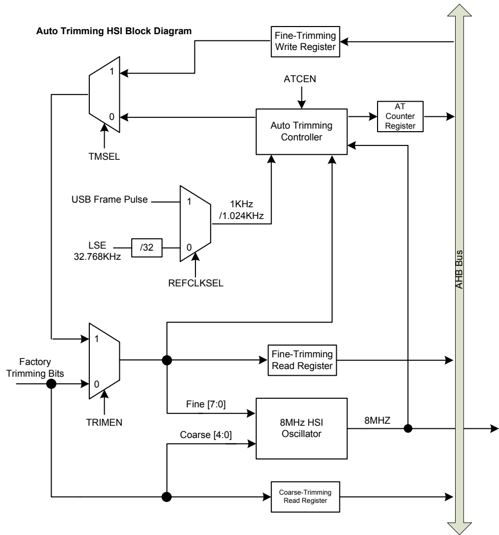
Figure 15. HSI Auto Trimming Block Diagram
