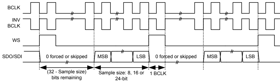
Figure 213. Right-justified Mono Mode Waveforms (32-bit Channel Enabled)
