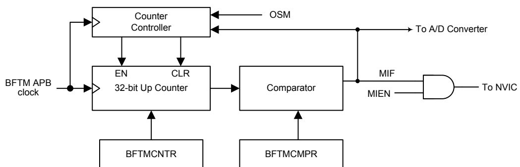
Figure 69. BFTM Block Diagram
