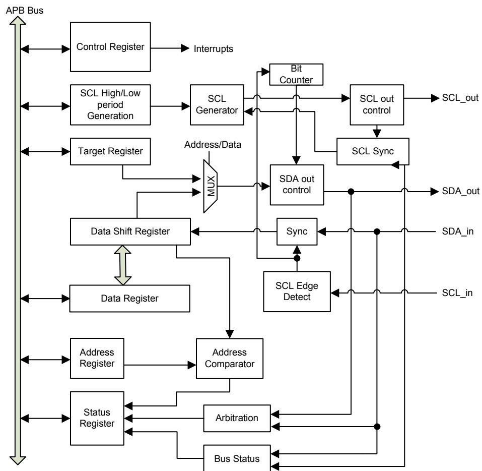
Figure 136. I 2 C Module Block Diagram
