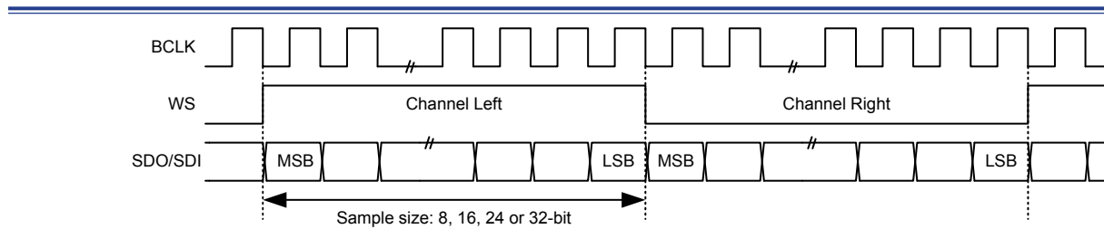
Figure 206. Right-justified Stereo Mode Waveforms
