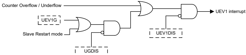
Figure 105. Update Event 1 Setup Diagram
