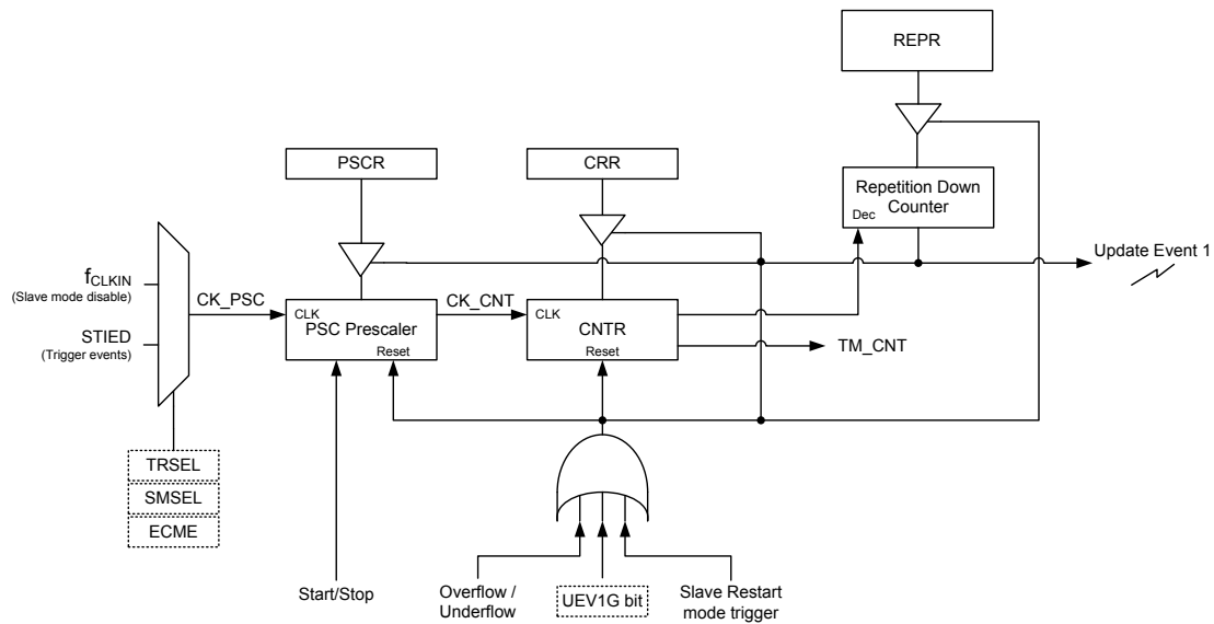
Figure 78. MCTM Clock Selection Source
