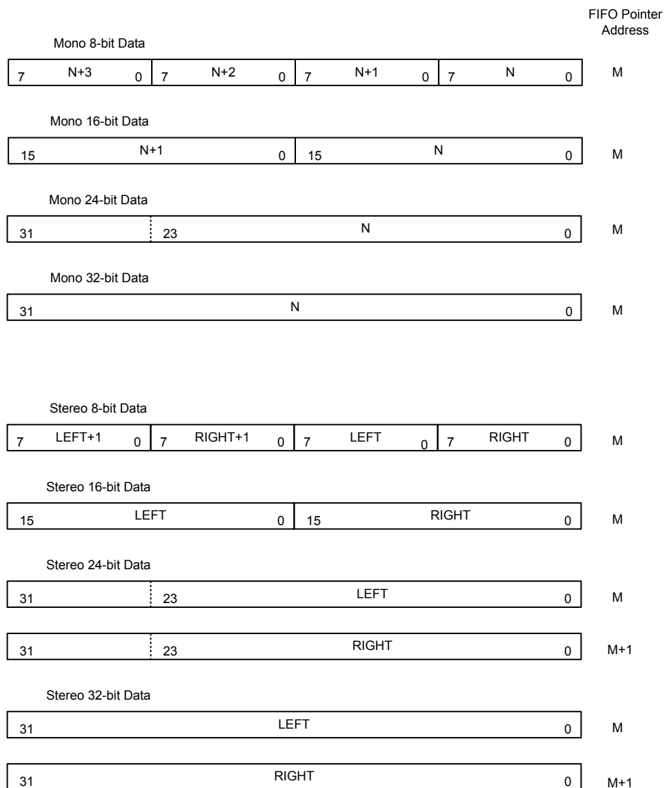
Figure 216. FIFO Data Content Arrangement for Various Modes
