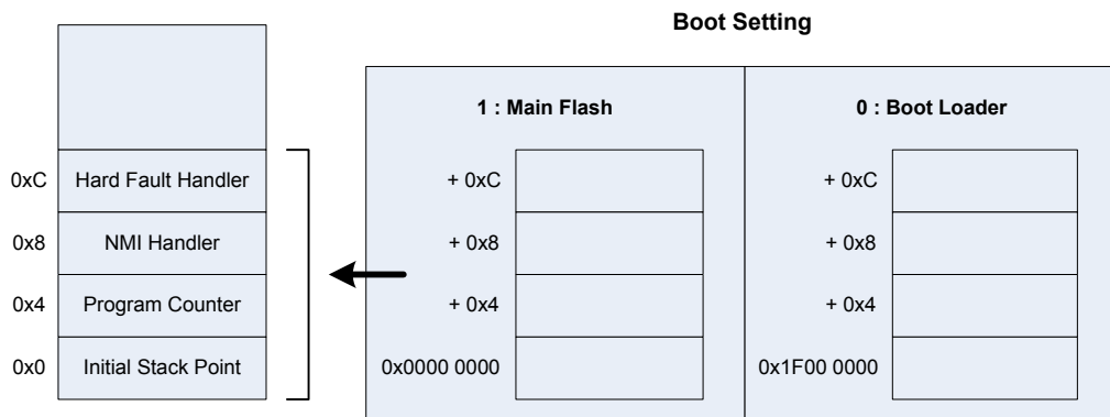
Figure 7. Vector Remapping
