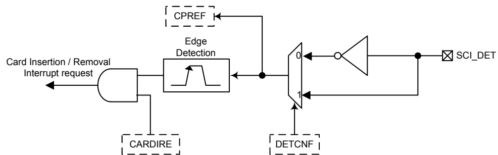
Figure 178. SCI Card Detection Diagram
