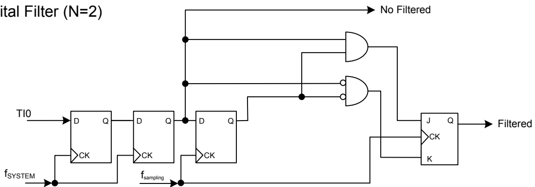
Figure 52. T10 Digital Filter Diagram with N = 2
