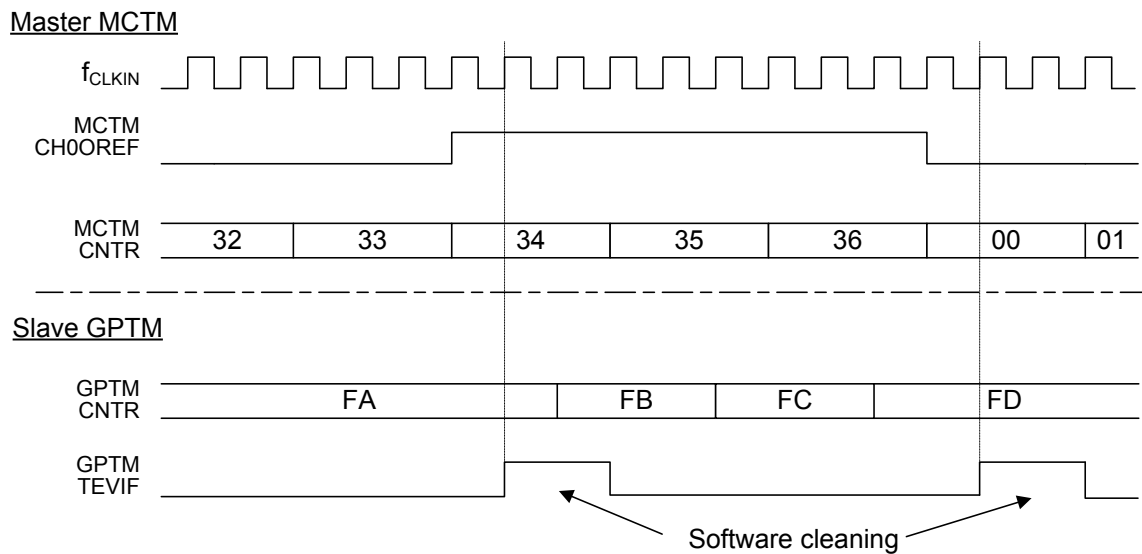
Figure 111. Pausing GPTM using the MCTM CH0OREF Signal
