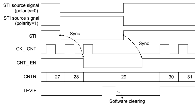
Figure 43. GPTM in Pause Mode
