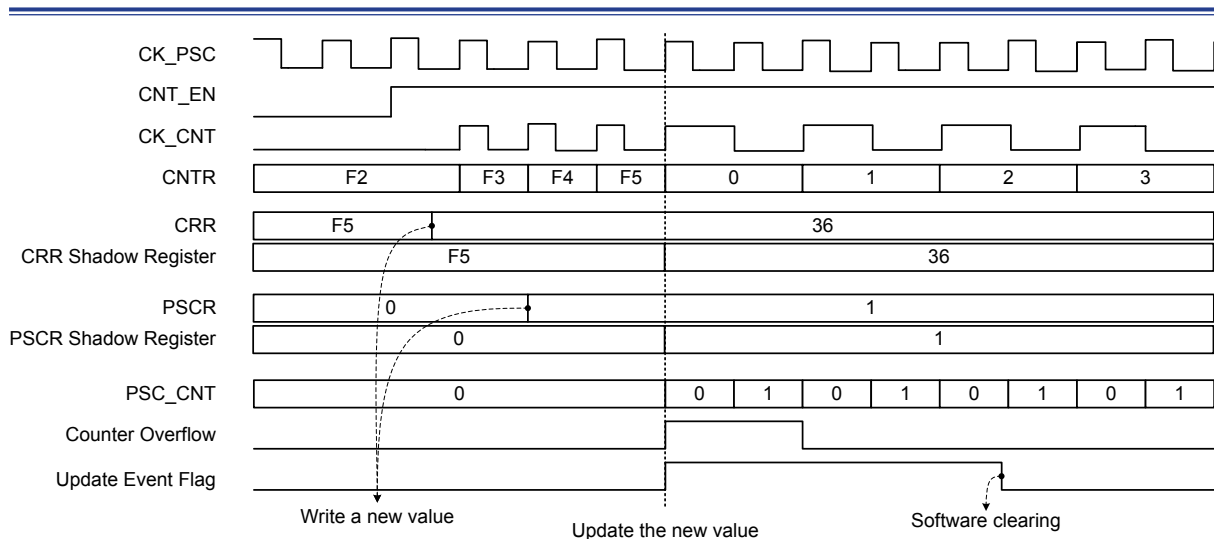
Figure 117. Up-counting Example
