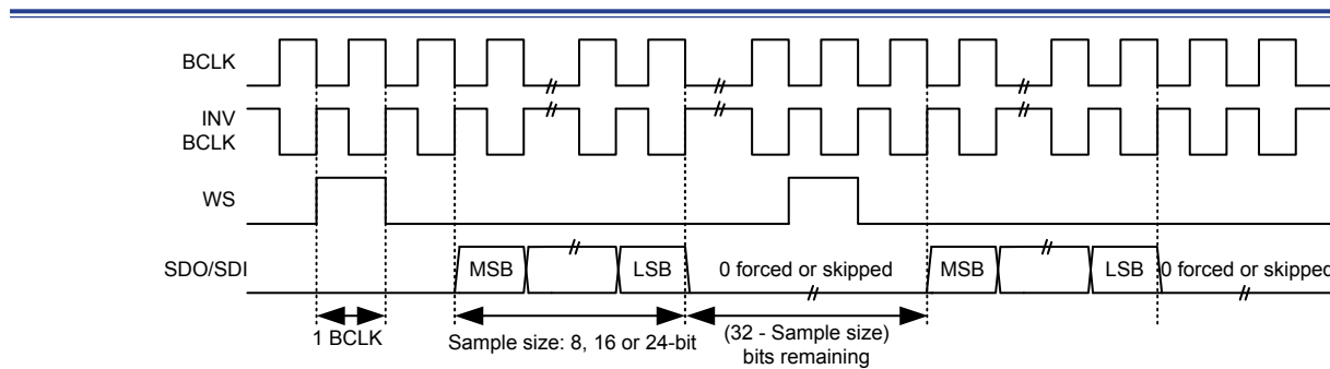
Figure 209. I 2 S-justified Mono Mode Waveforms (32-bit Channel Enabled)
