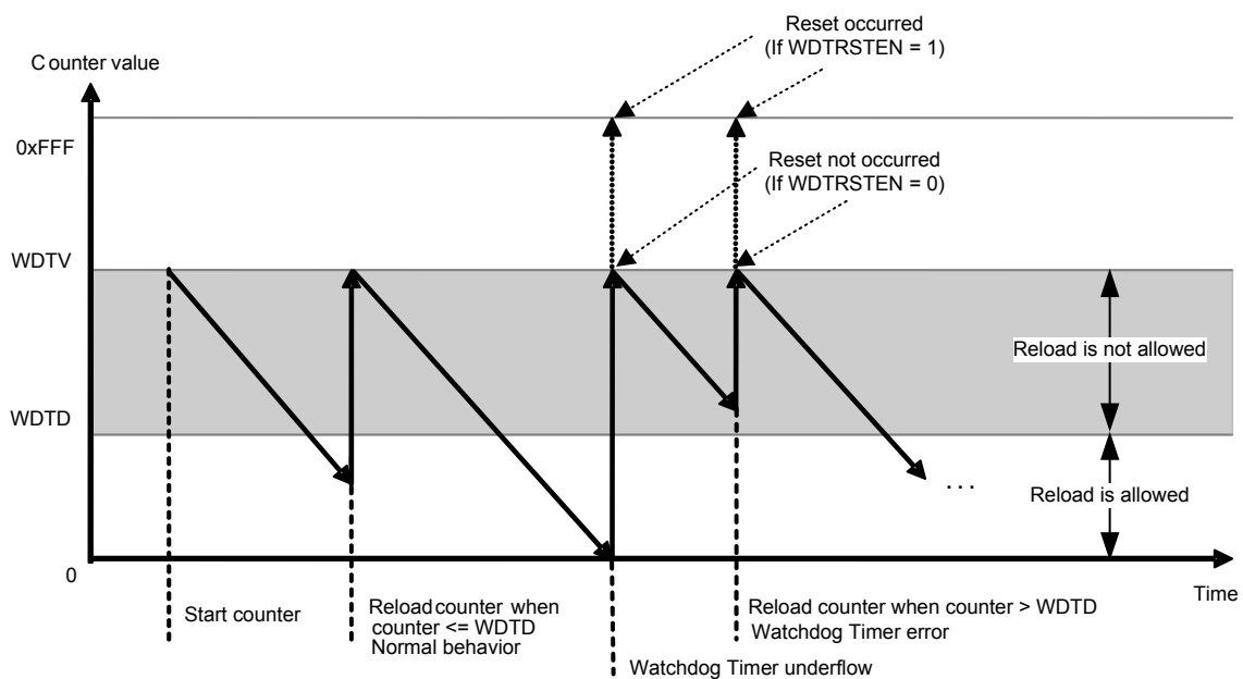
Figure 135. Watchdog Timer Behavior
