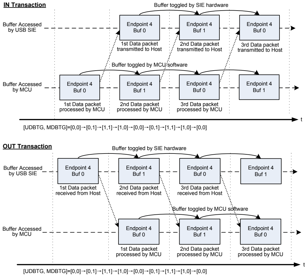
Figure 182. Double-buffering Operation Example
