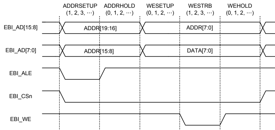
Figure 195. EBI Multiplexed 8-bit Data, 20-bit Address Write Operation
