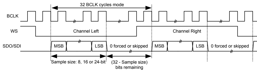
Figure 203. I 2 S-justified Stereo Mode Waveforms (32-bit Channel Enabled)
