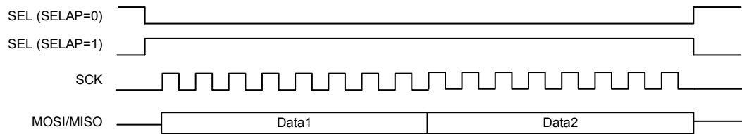
Figure 154. SPI Continuous Transfer Timing Diagram – CPOL = 0, CPHA = 1
