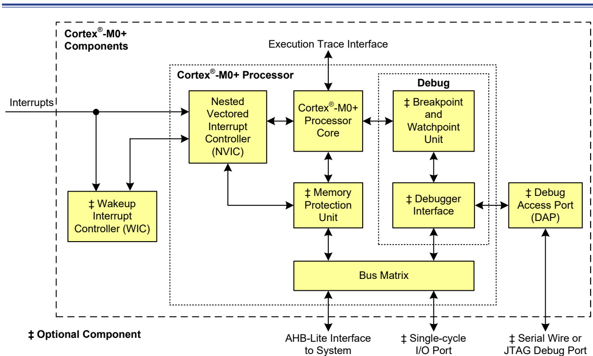
Figure 2. Cortex-M0+ Block Diagram
