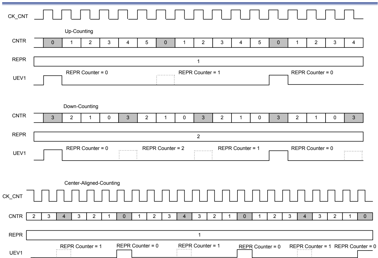
Figure 77. Update Event 1 Dependent Repetition Mechanism Example
