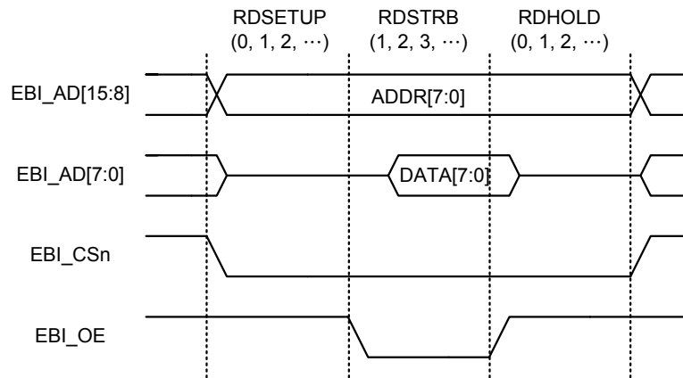
Figure 187. EBI Non-multiplexed 8-bit Data, 8-bit Address Read Operation
