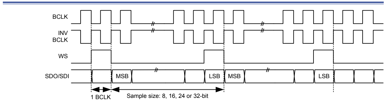
Figure 210. Left-justified Mono Mode Waveforms
