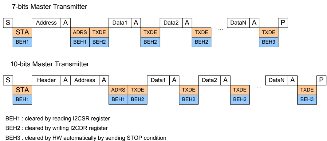
Figure 145. Master Transmitter Timing Diagram
