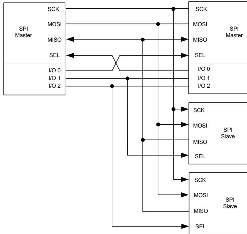
Figure 159. SPI Multi-Master Slave Environment
