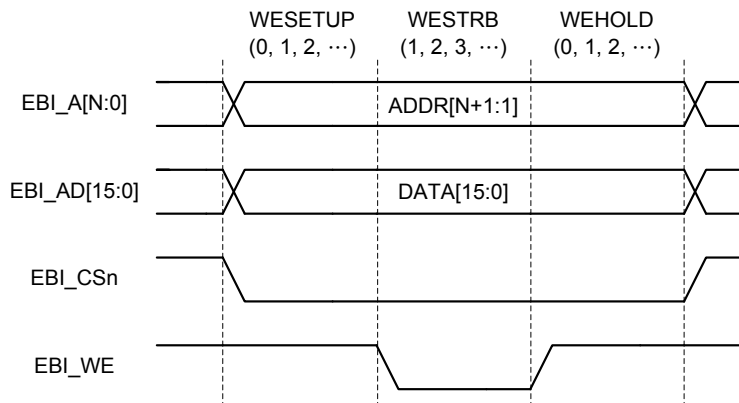
Figure 190. EBI Non-multiplexed 16-bit Data, N-bit Address Write Operation
