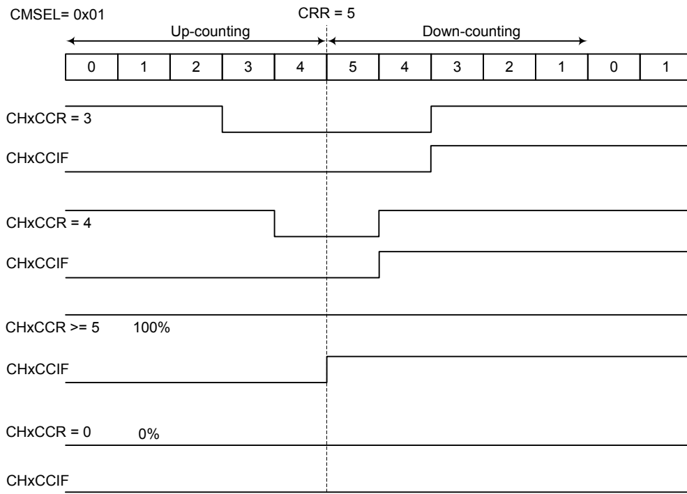
Figure 97. PWM Mode 1 Channel Output Reference Signal and Counter in Centre-aligned Counting Mode
