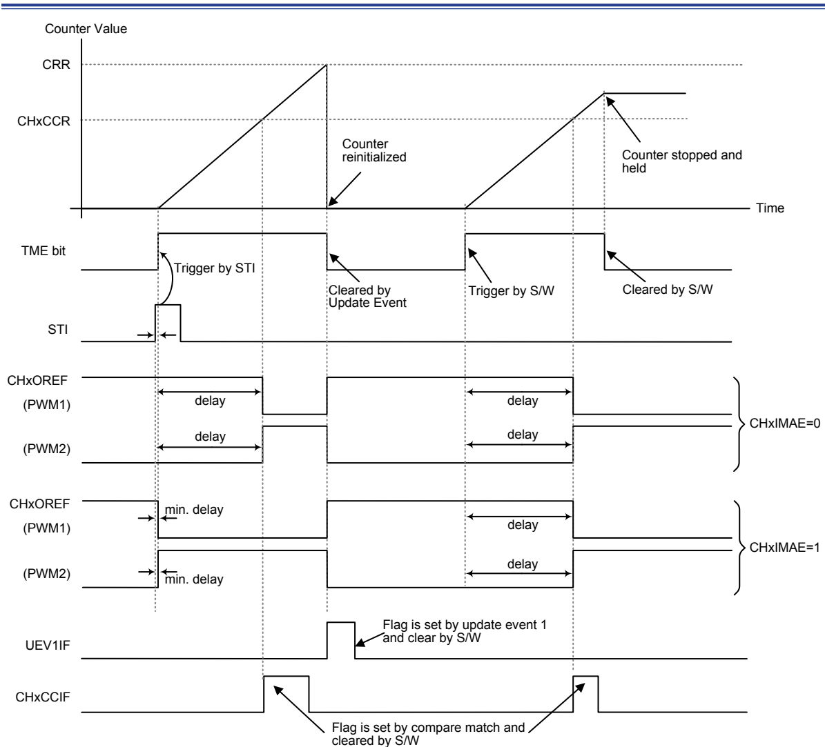
Figure 62. Single Pulse Mode
