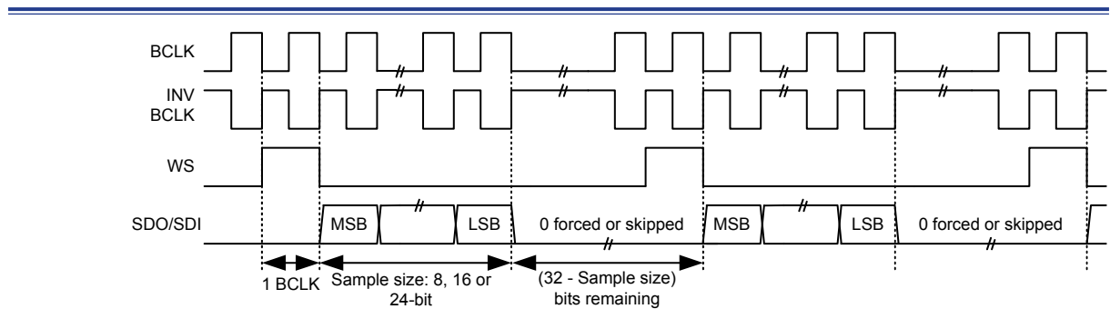
Figure 211. Left-justified Mono Mode Waveforms (32-bit Channel Enabled)
