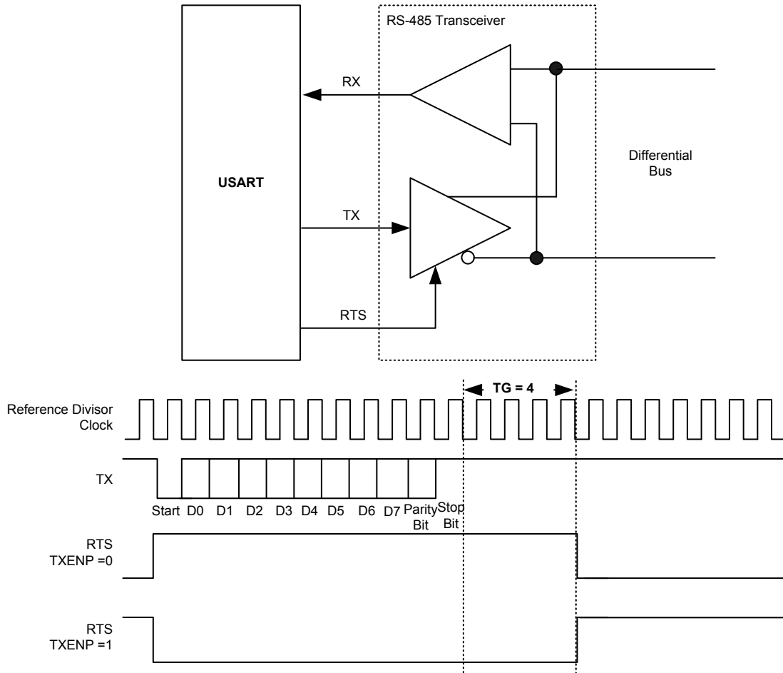
Figure 168. RS485 Interface and Waveform
