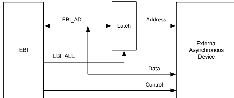
Figure 191. An EBI Address Latch Setup Diagram
