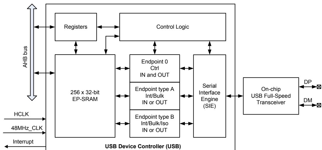
Figure 180. USB Block Diagram
