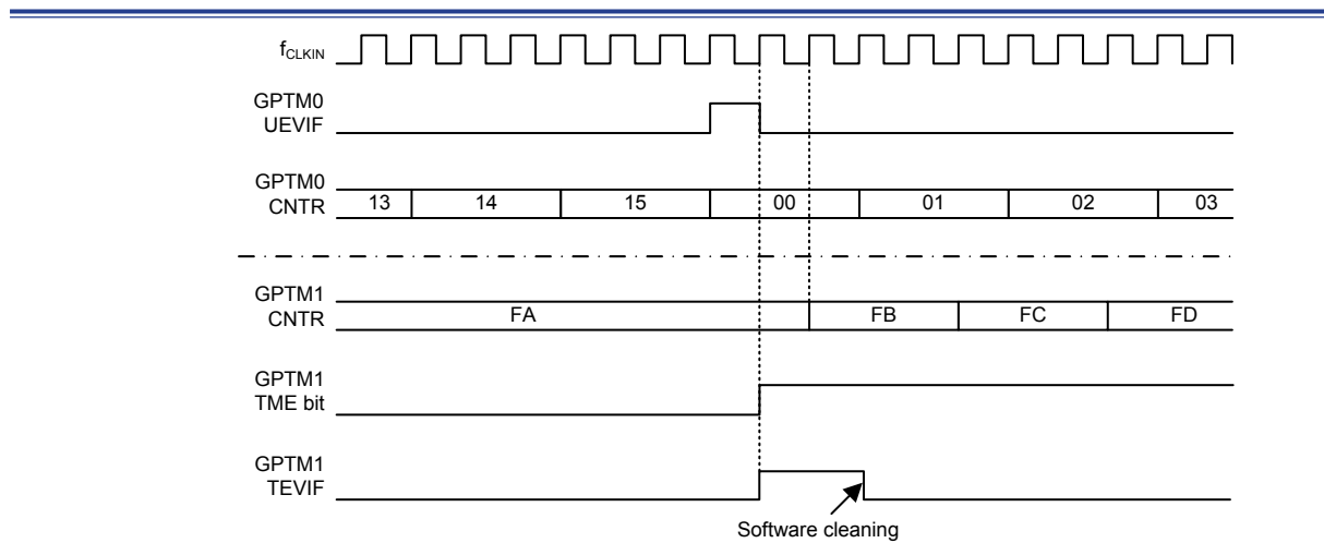
Figure 66. Triggering GPTM1 with GPTM0 Update Event
