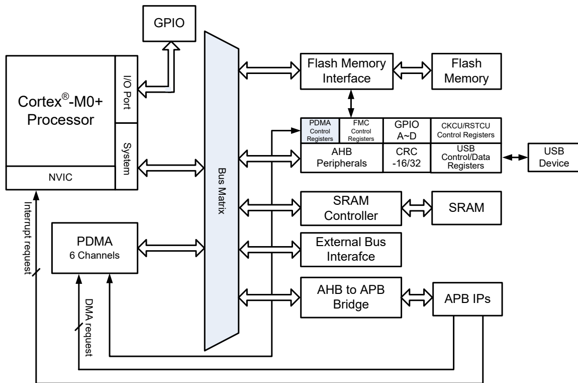
Figure 3. Bus Architecture
