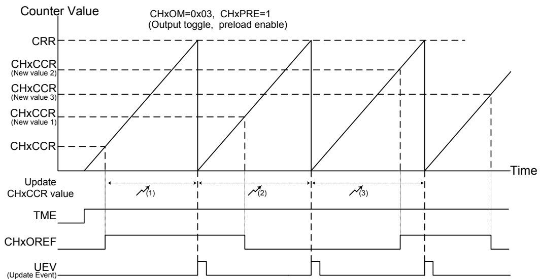
Figure 57. Toggle Mode Channel Output Reference Signal (CHxPRE = 1)
