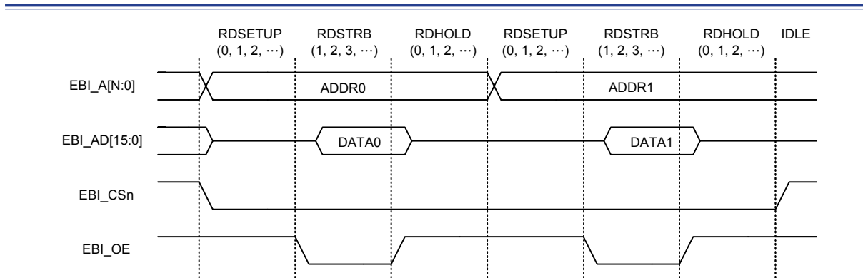
Figure 197. EBI De-asserts an IDLE Cycle between Transactions in the Same Bank (NOIDLE = 1)
