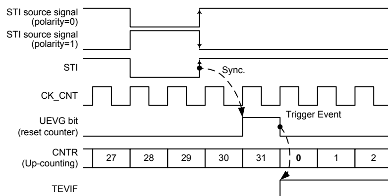
Figure 121. SCTM in Restart Mode
