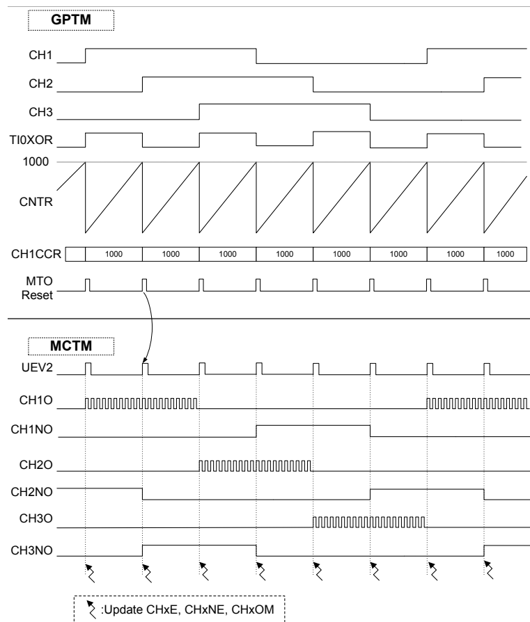
Figure 114. CH1XOR Input as Hall Sensor Interface
