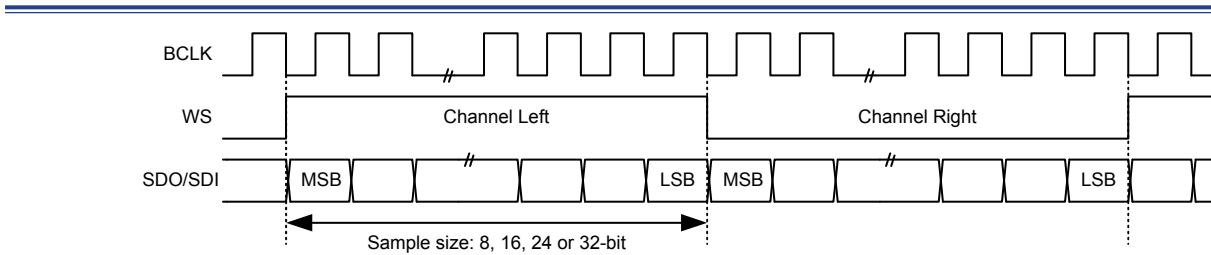
Figure 204. Left-justified Stereo Mode Waveforms
