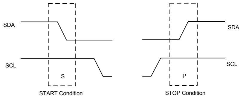
Figure 137. START and STOP Condition
