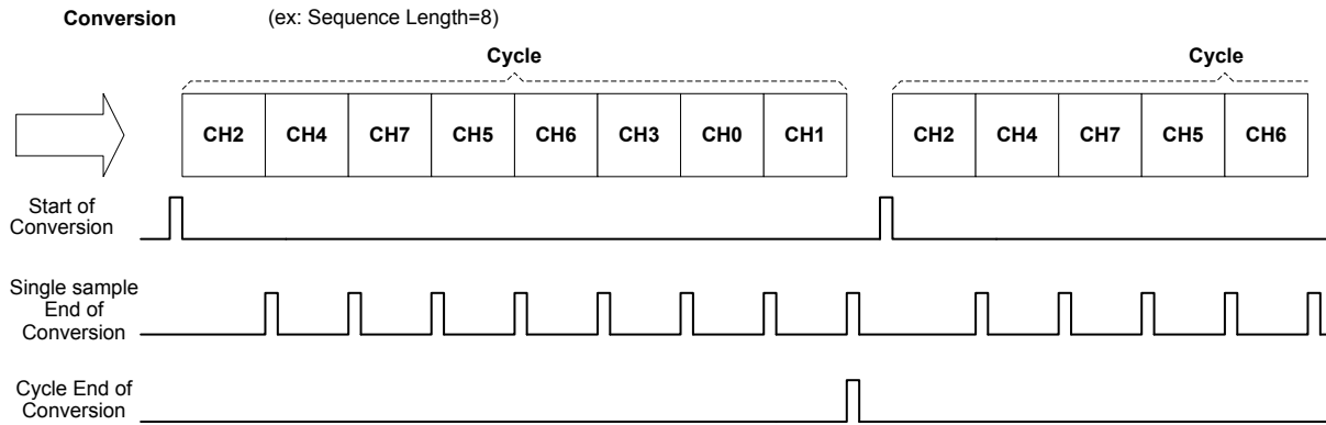
Figure 28. One Shot Conversion Mode
