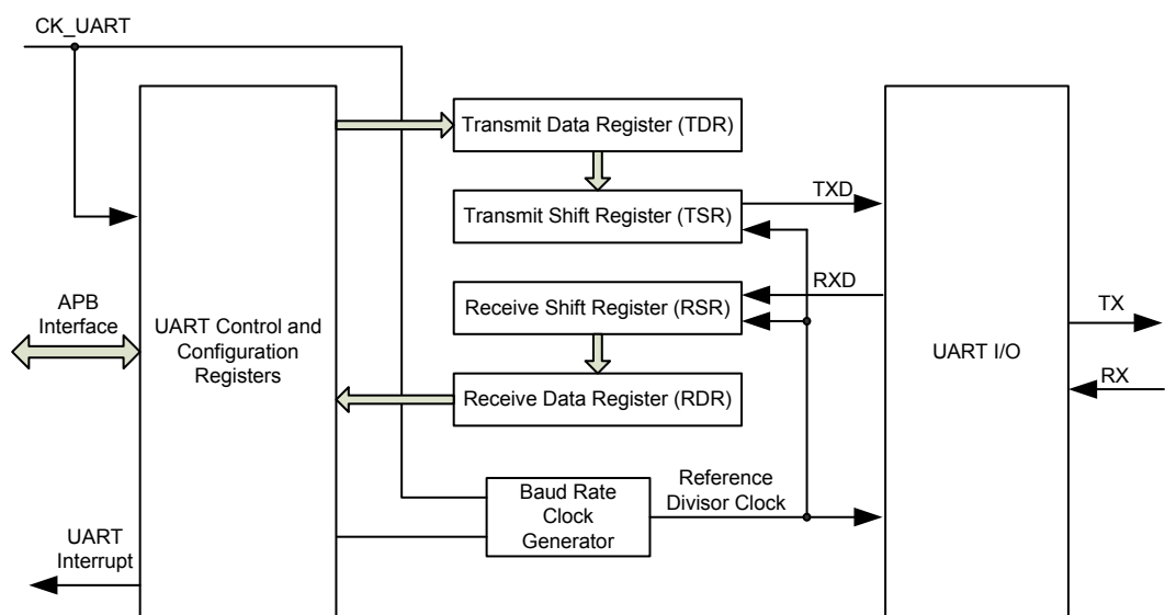
Figure 171. UART Block Diagram
