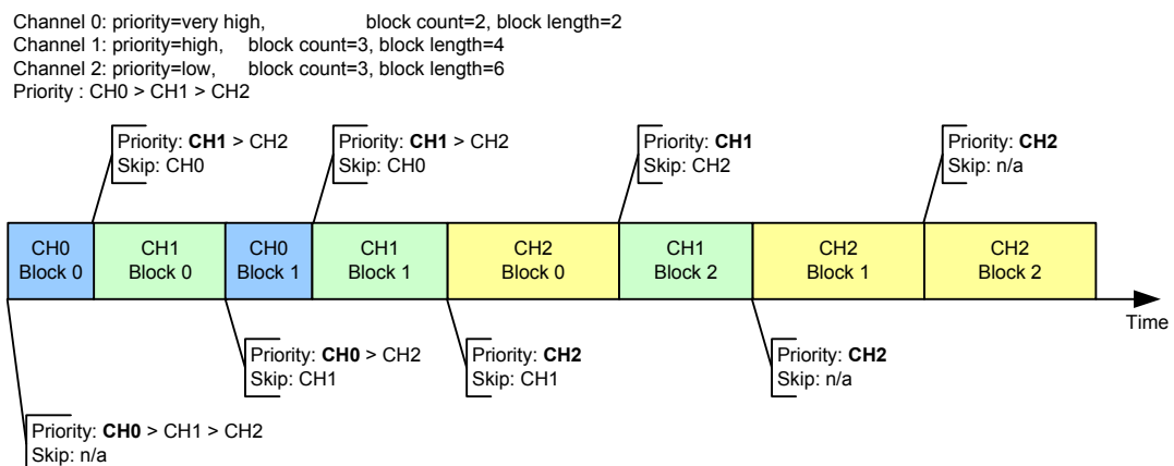
Figure 185. PDMA Channel Arbitration and Scheduling Example
