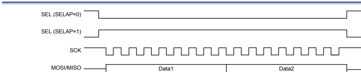
Figure 158. SPI Continuous Transfer Timing Diagram – CPOL = 1, CPHA = 1
