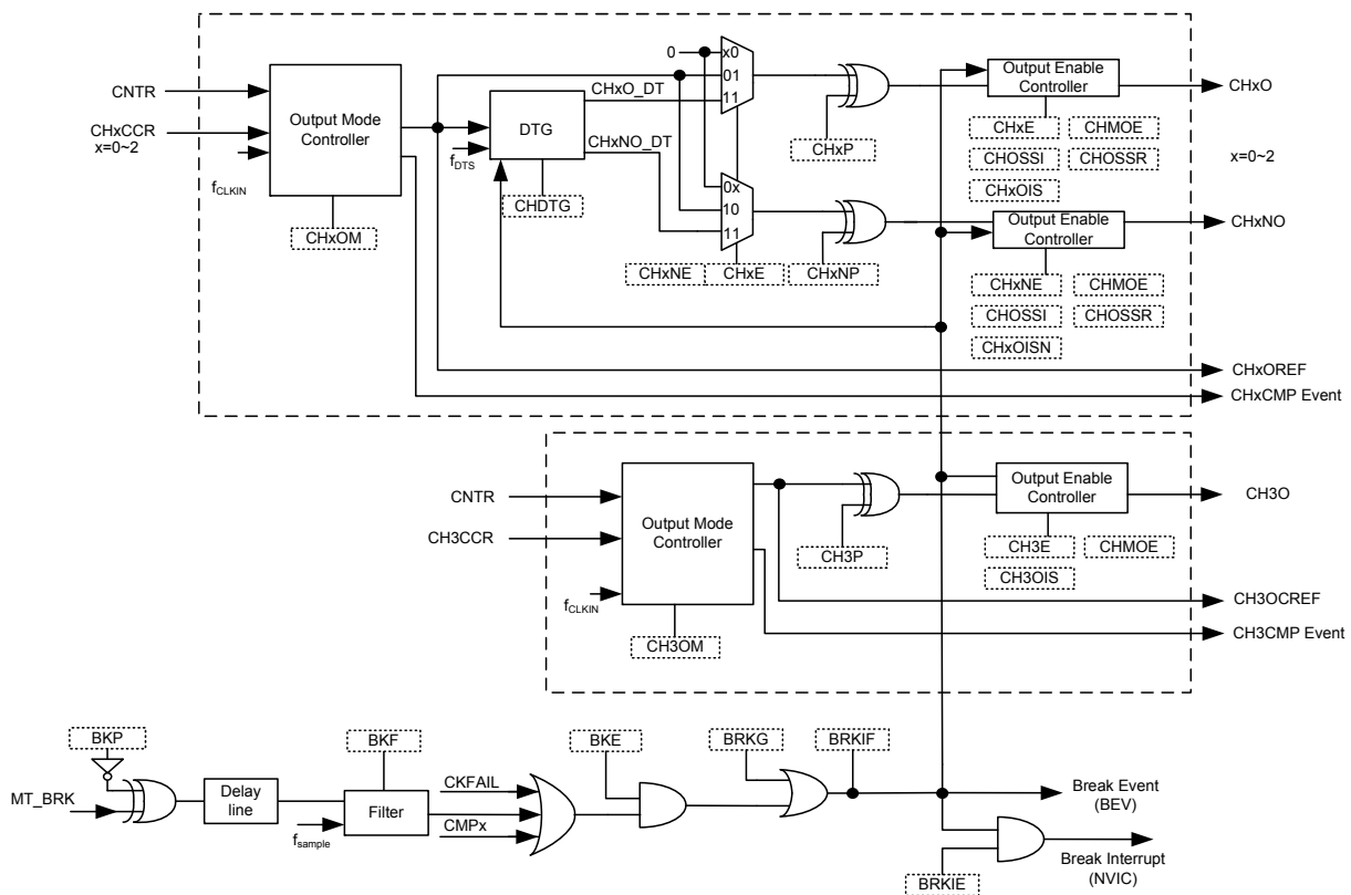
Figure 92. Output Stage Block Diagram
