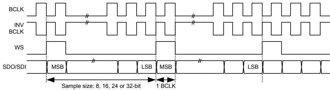
Figure 212. Right-justified Mono Mode Waveforms
