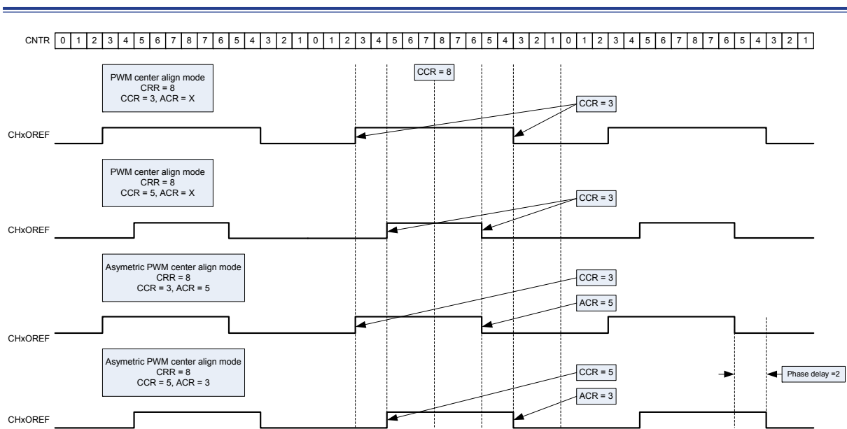
Figure 64. Asymmetric PWM mode versus center align counting mode
