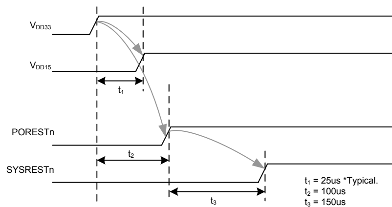
Figure 19. Power On Reset Sequence
