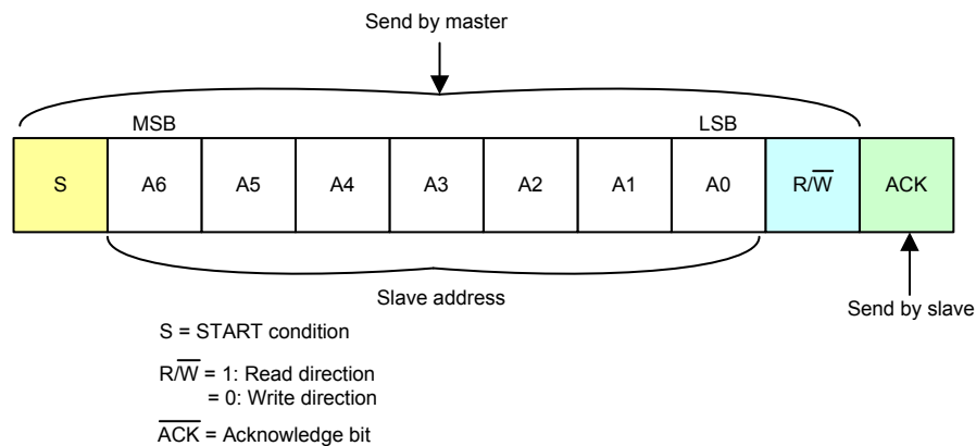
Figure 139. 7-bit Addressing Mode
