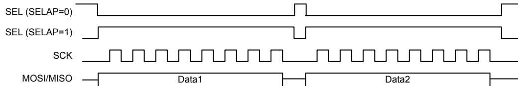
Figure 152. SPI Continuous Data Transfer Timing Diagram – CPOL = 0, CPHA = 0
