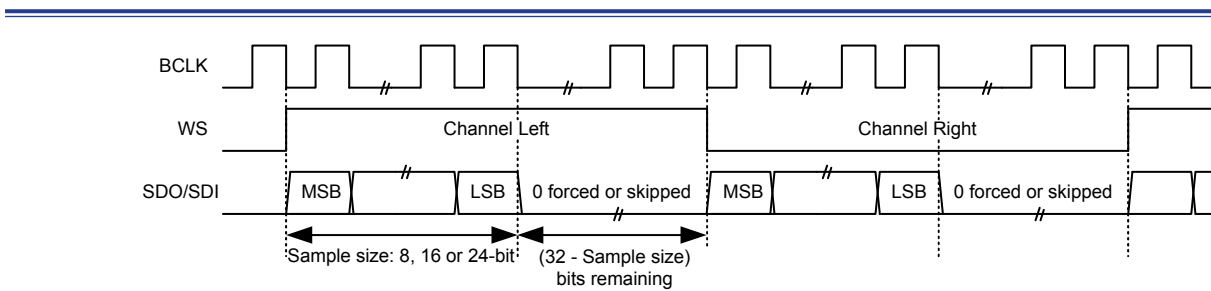
Figure 205. Left-justified Stereo Mode Waveforms (32-bit Channel Enabled)
