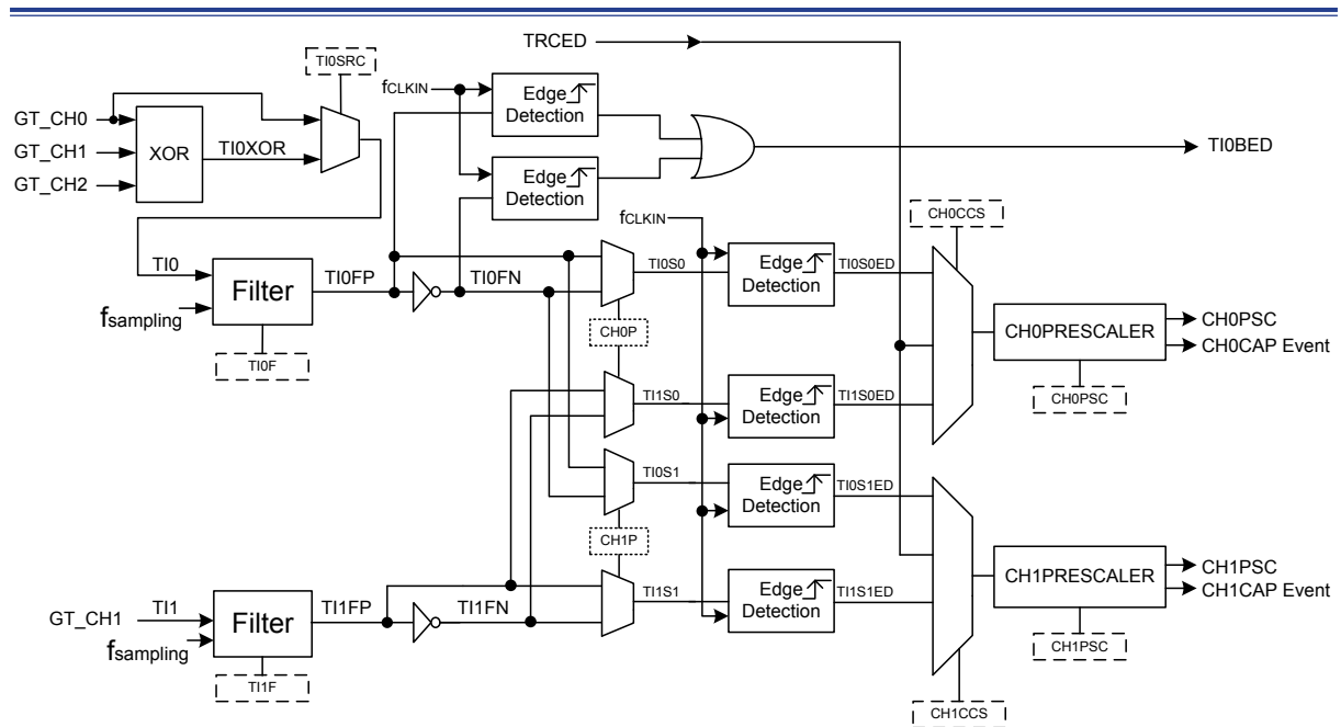
Figure 50. Channel 0 and Channel 1 Input Stages
