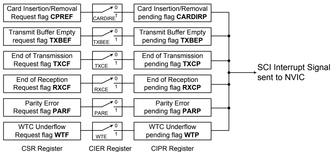
Figure 179. SCI Interrupt Structure
