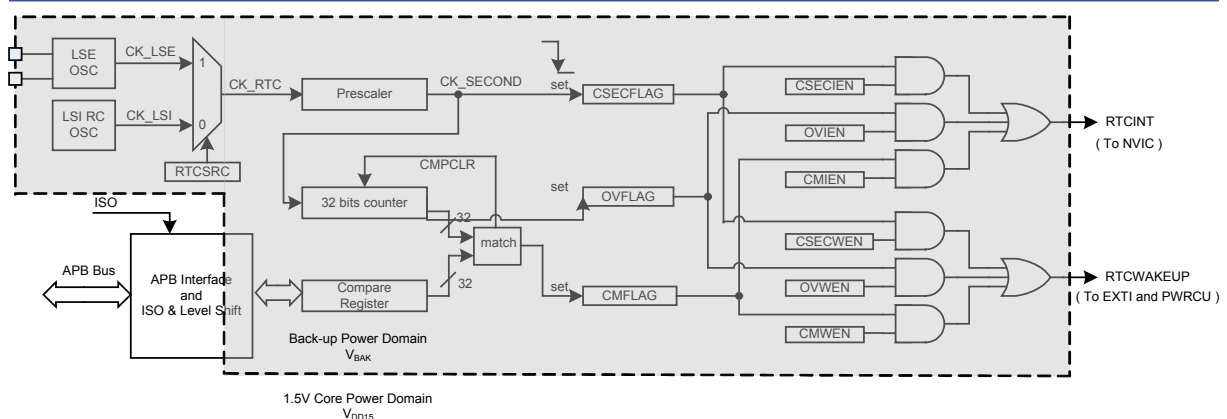
Figure 133. RTC Block Diagram
