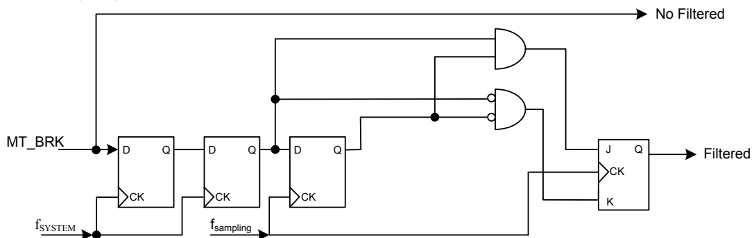
Figure 100. MT_BRK Pin Digital Filter Diagram with N = 2
