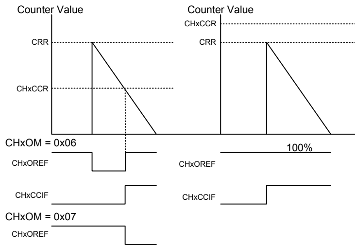
Figure 59. PWM Mode Channel Output Reference Signal and Counter in Down-counting Mode
