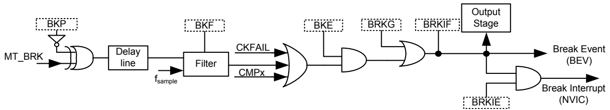
Figure 99. MCTM Break Signal Block Diagram
