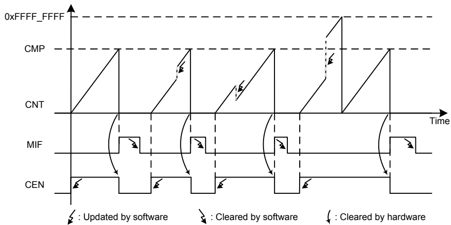
Figure 72. BFTM – One Shot Mode Counter Updating
