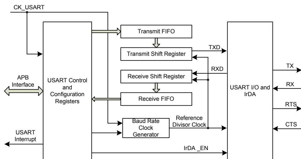
Figure 160. USART Block Diagram
