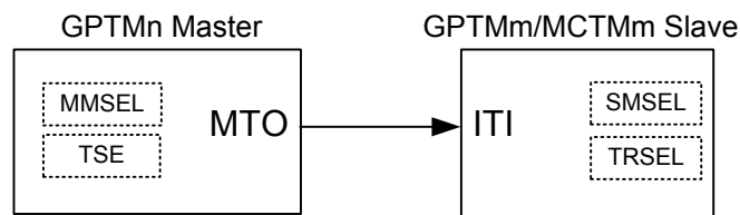
Figure 45. Master GPTMn and Slave GPTMm/MCTMm Connection
