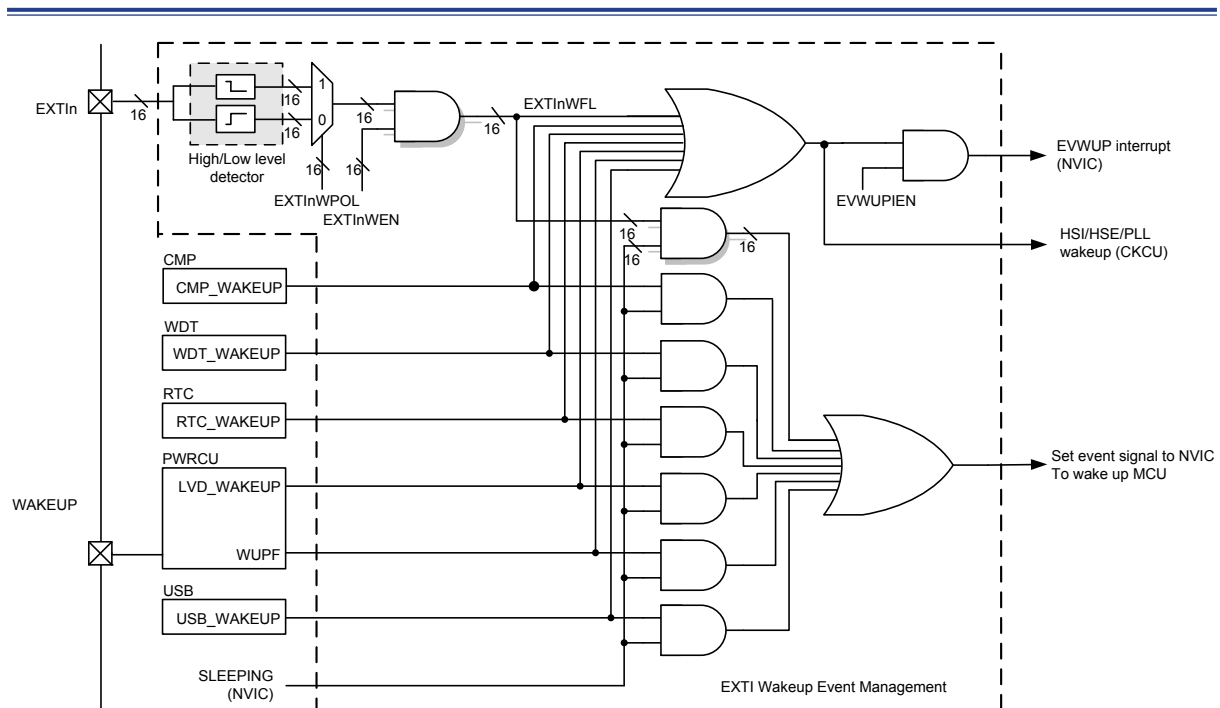
Figure 25. EXTI Wake-up Event Management
