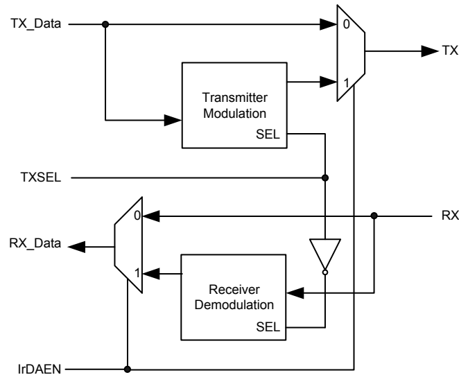
Figure 167. USART I/O and IrDA Block Diagram
