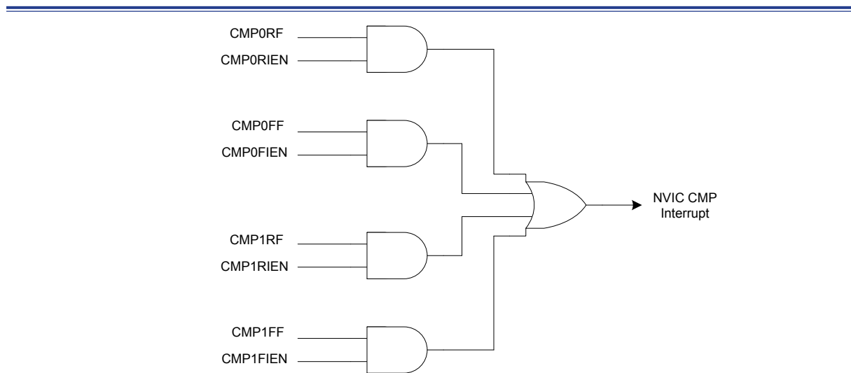
Figure 33. Interrupt Signals of Comparators
