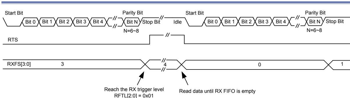
Figure 164. USART RTS Flow Control
