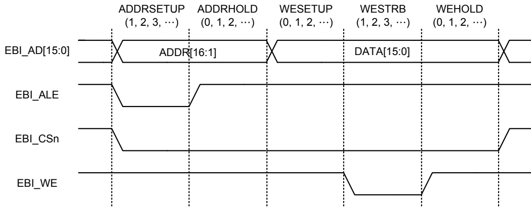
Figure 193. EBI Multiplexed 16-bit Data, 16-bit Address Write Operation
