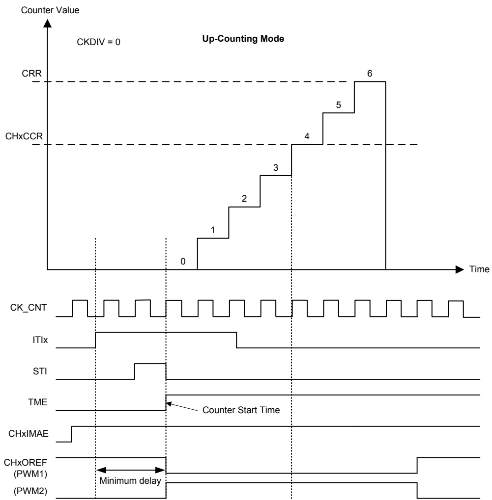
Figure 109. Immediate Active Mode Minimum Delay
