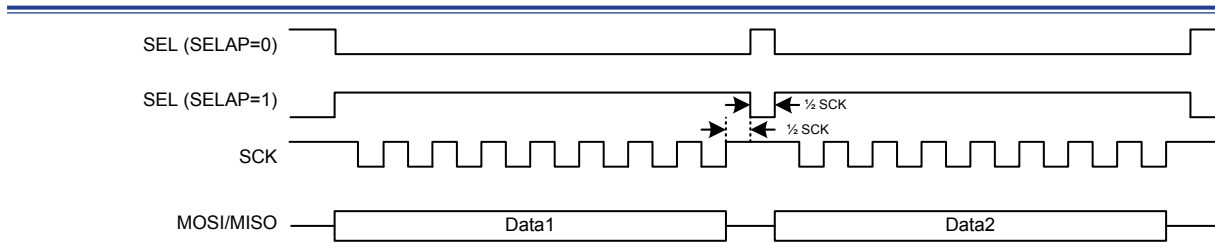
Figure 156. SPI Continuous Transfer Timing Diagram – CPOL = 1, CPHA = 0
