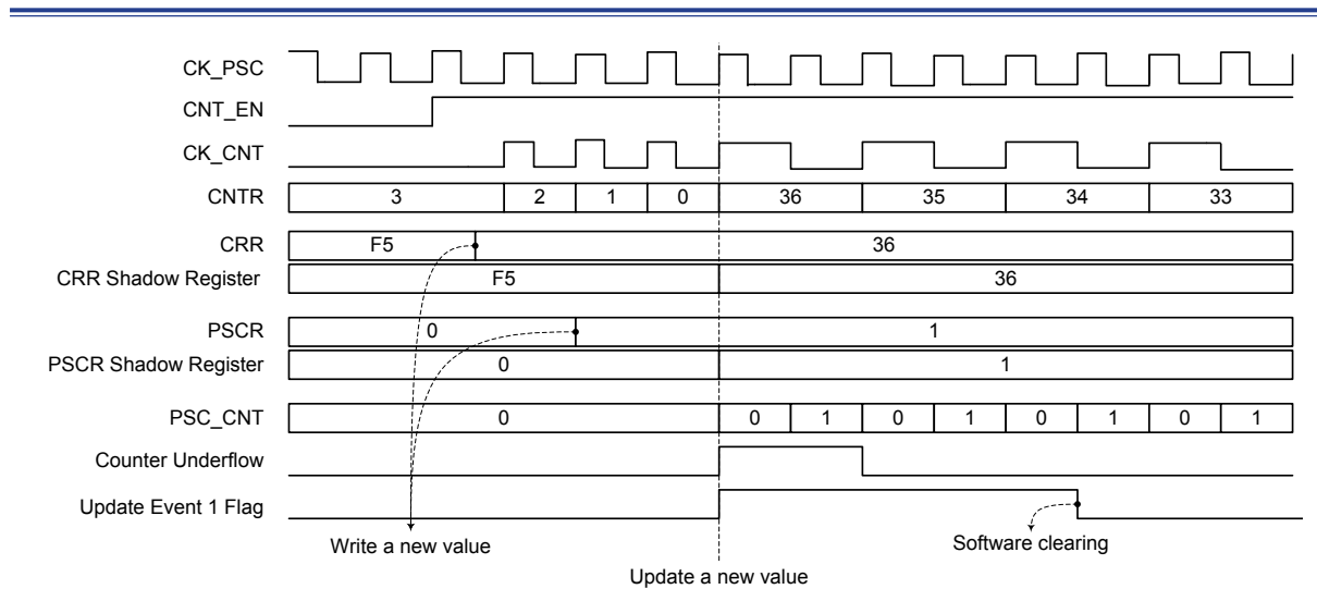
Figure 75. Down-counting Example
