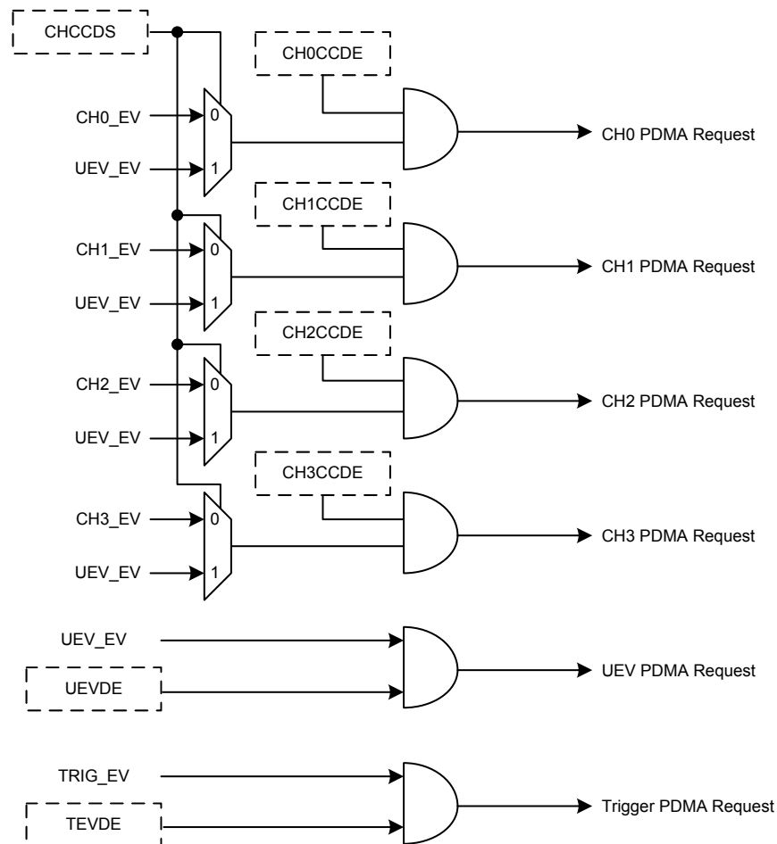
Figure 68. GPTM PDMA Mapping Diagram
