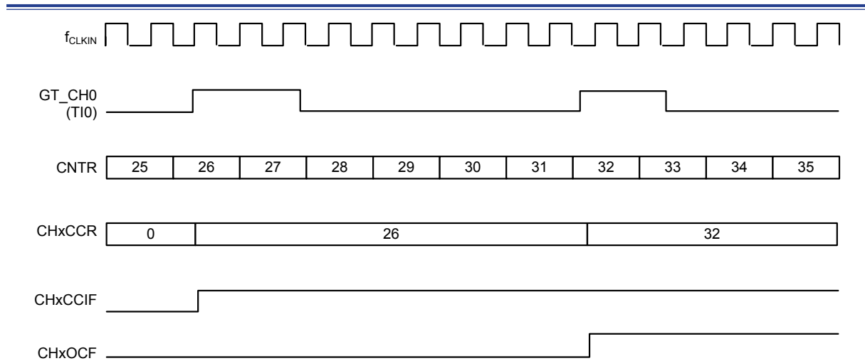
Figure 48. Input Capture Mode
