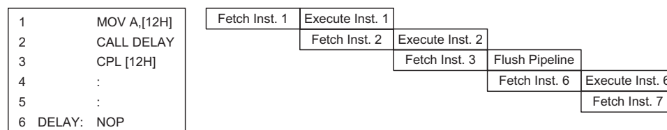
Instruction Fetching
