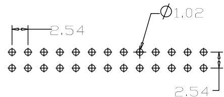
PCB LAYOUT
