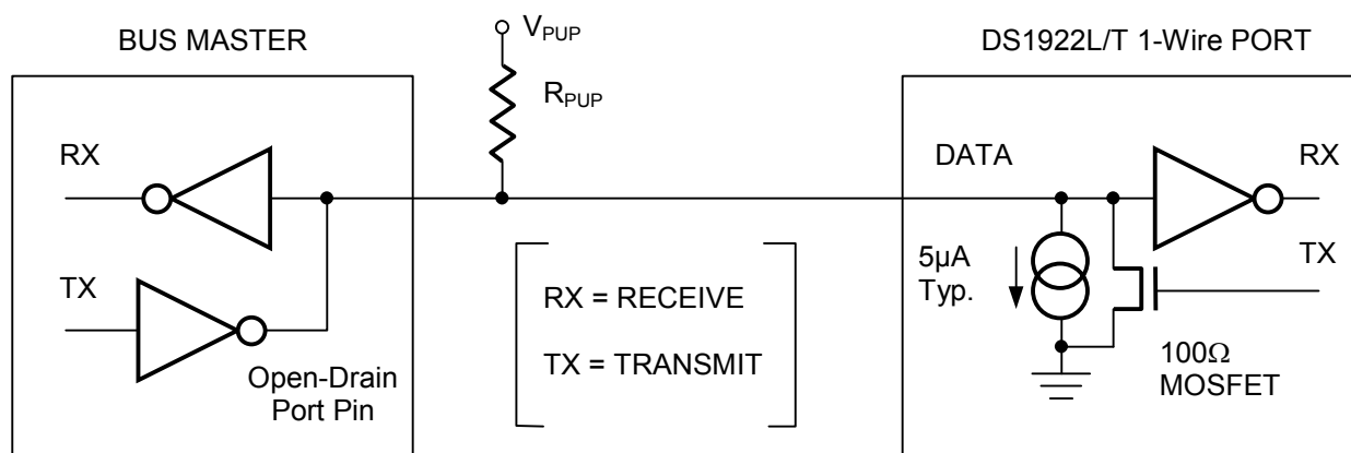
Figure 10. Hardware Configuration
